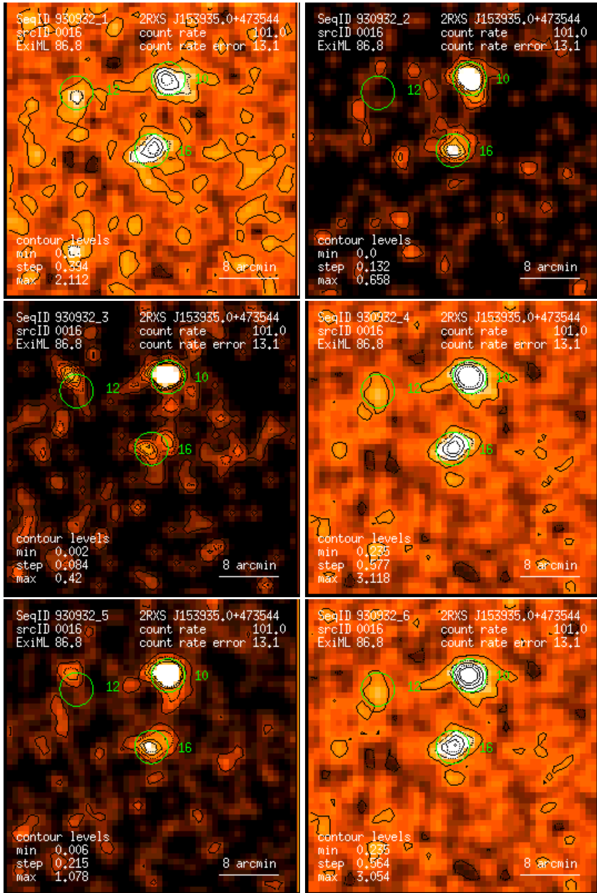
Figure 16: RASS 930932: detection 0016: band rate images, Gaussian filter: (1) PSPC channels 11 – 41, (2) 52 – 90, (3) 91 – 201, (4) 11 – 235, (5) 52 – 201, (6) 11 – 201. Broad band rates in counts/ks. Band rate contour levels in counts/ks/arcmin 2 .
