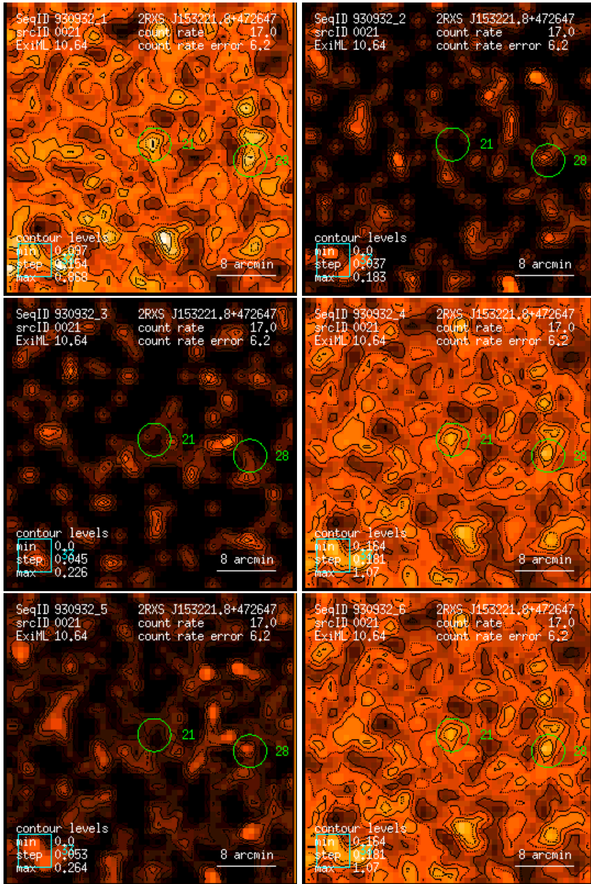
Figure 21: RASS 930932: detection 0021: band rate images, Gaussian filter: (1) PSPC channels 11 – 41, (2) 52 – 90, (3) 91 – 201, (4) 11 – 235, (5) 52 – 201, (6) 11 – 201. Broad band rates in counts/ks. Band rate contour levels in counts/ks/arcmin 2 .
