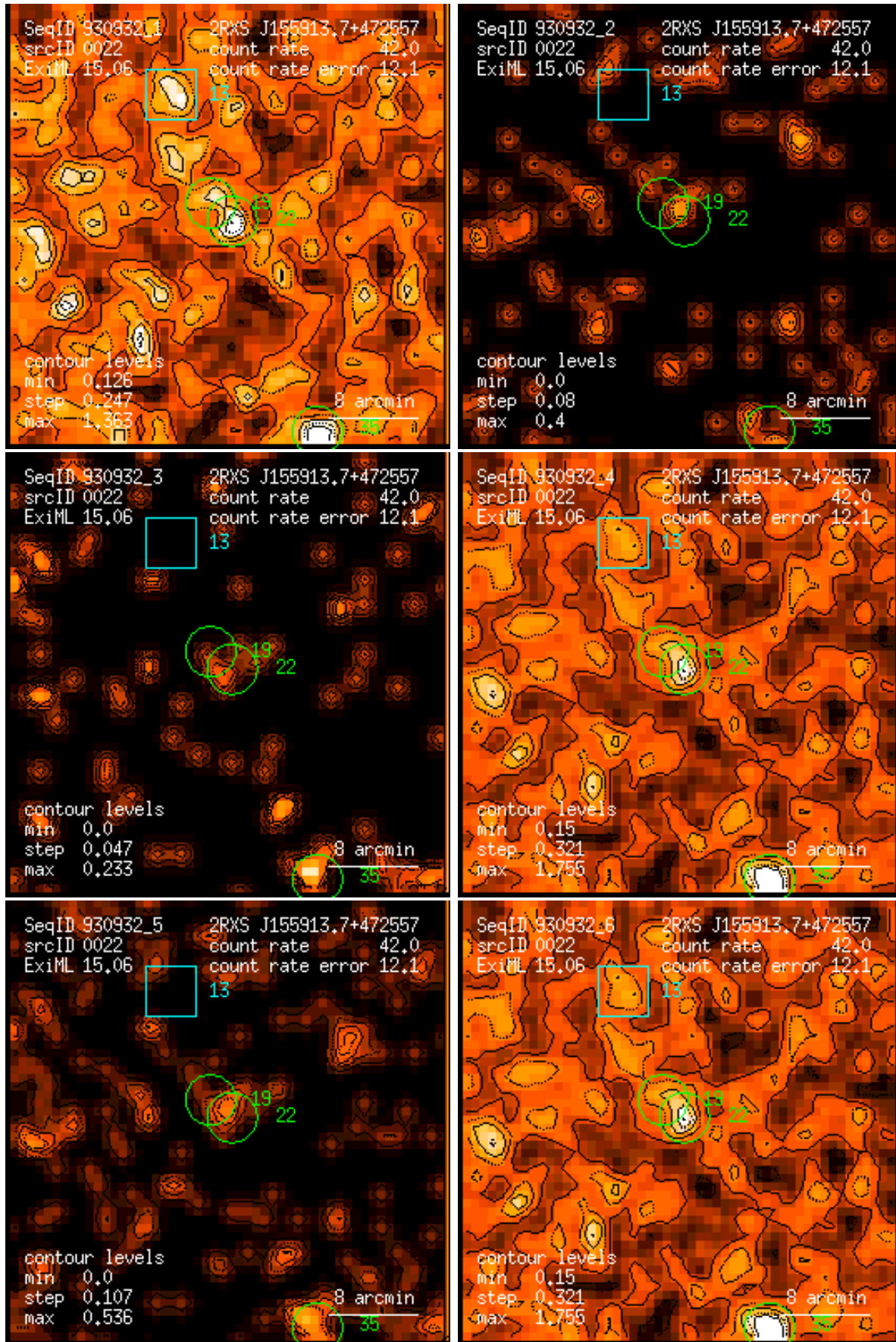
Figure 22: RASS 930932: detection 0022: band rate images, Gaussian filter: (1) PSPC channels 11 – 41, (2) 52 – 90, (3) 91 – 201, (4) 11 – 235, (5) 52 – 201, (6) 11 – 201. Broad band rates in counts/ks. Band rate contour levels in counts/ks/arcmin 2 .
