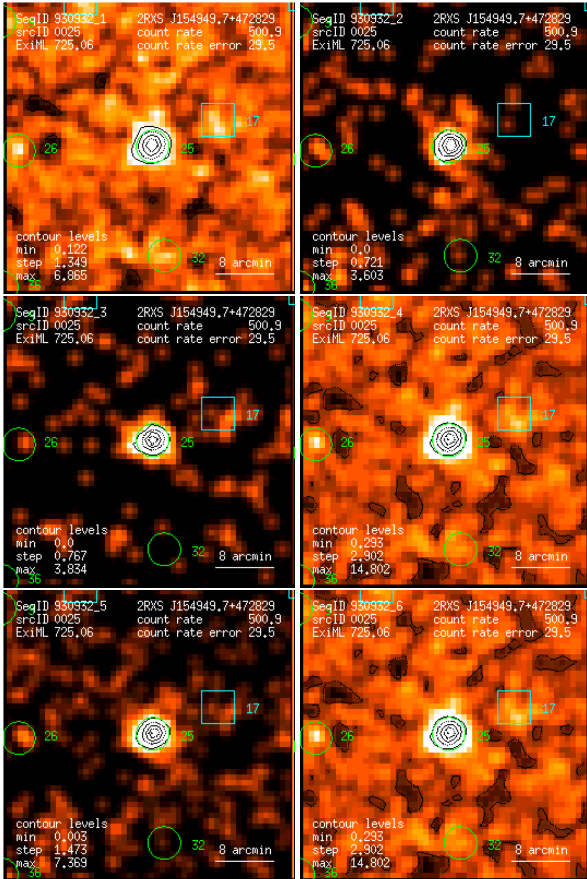
Figure 25: RASS 930932: detection 0025: band rate images, Gaussian filter: (1) PSPC channels 11 – 41, (2) 52 – 90, (3) 91 – 201, (4) 11 – 235, (5) 52 – 201, (6) 11 – 201. Broad band rates in counts/ks. Band rate contour levels in counts/ks/arcmin 2 .
