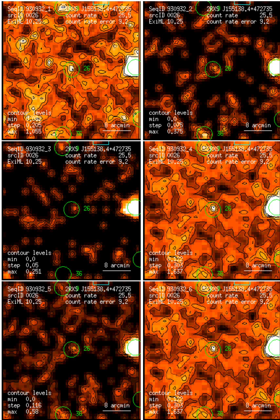
Figure 26: RASS 930932: detection 0026: band rate images, Gaussian filter: (1) PSPC channels 11 – 41, (2) 52 – 90, (3) 91 – 201, (4) 11 – 235, (5) 52 – 201, (6) 11 – 201. Broad band rates in counts/ks. Band rate contour levels in counts/ks/arcmin 2 .
