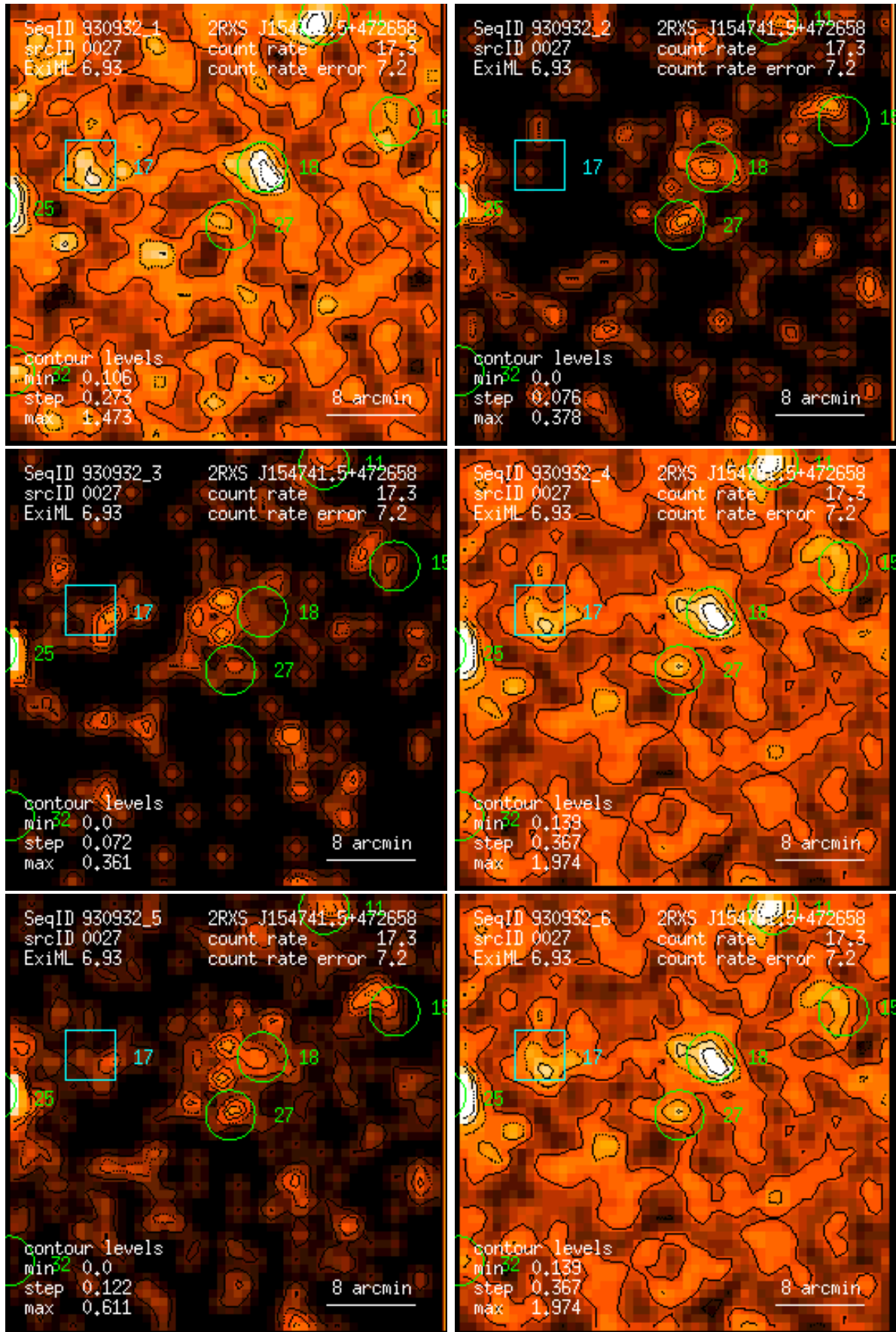
Figure 27: RASS 930932: detection 0027: band rate images, Gaussian filter: (1) PSPC channels 11 – 41, (2) 52 – 90, (3) 91 – 201, (4) 11 – 235, (5) 52 – 201, (6) 11 – 201. Broad band rates in counts/ks. Band rate contour levels in counts/ks/arcmin 2 .
