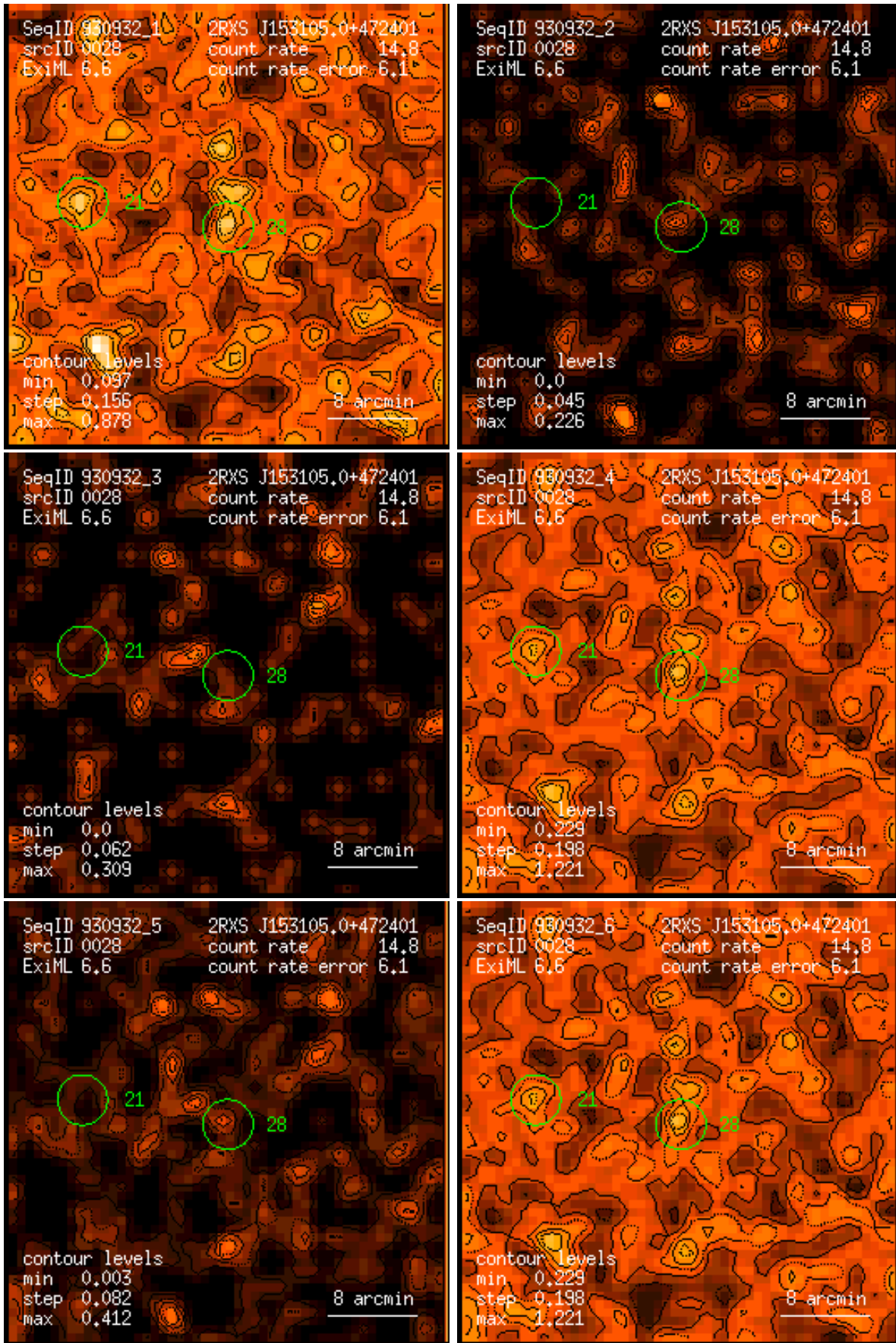
Figure 28: RASS 930932: detection 0028: band rate images, Gaussian filter: (1) PSPC channels 11 – 41, (2) 52 – 90, (3) 91 – 201, (4) 11 – 235, (5) 52 – 201, (6) 11 – 201. Broad band rates in counts/ks. Band rate contour levels in counts/ks/arcmin 2 .
