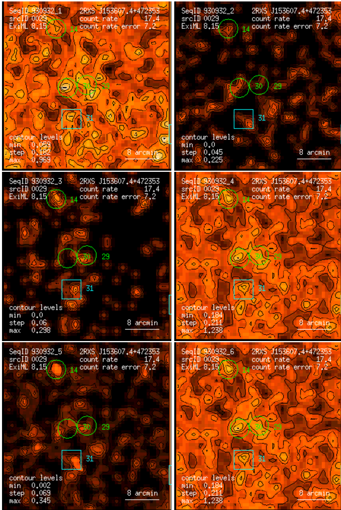
Figure 29: RASS 930932: detection 0029: band rate images, Gaussian filter: (1) PSPC channels 11 – 41, (2) 52 – 90, (3) 91 – 201, (4) 11 – 235, (5) 52 – 201, (6) 11 – 201. Broad band rates in counts/ks. Band rate contour levels in counts/ks/arcmin 2 .
