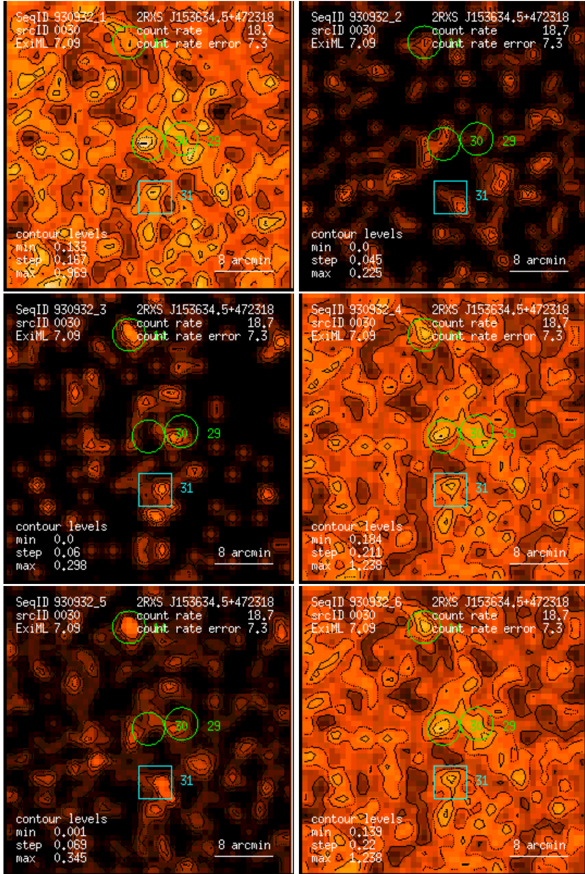
Figure 30: RASS 930932: detection 0030: band rate images, Gaussian filter: (1) PSPC channels 11 – 41, (2) 52 – 90, (3) 91 – 201, (4) 11 – 235, (5) 52 – 201, (6) 11 – 201. Broad band rates in counts/ks. Band rate contour levels in counts/ks/arcmin 2 .
