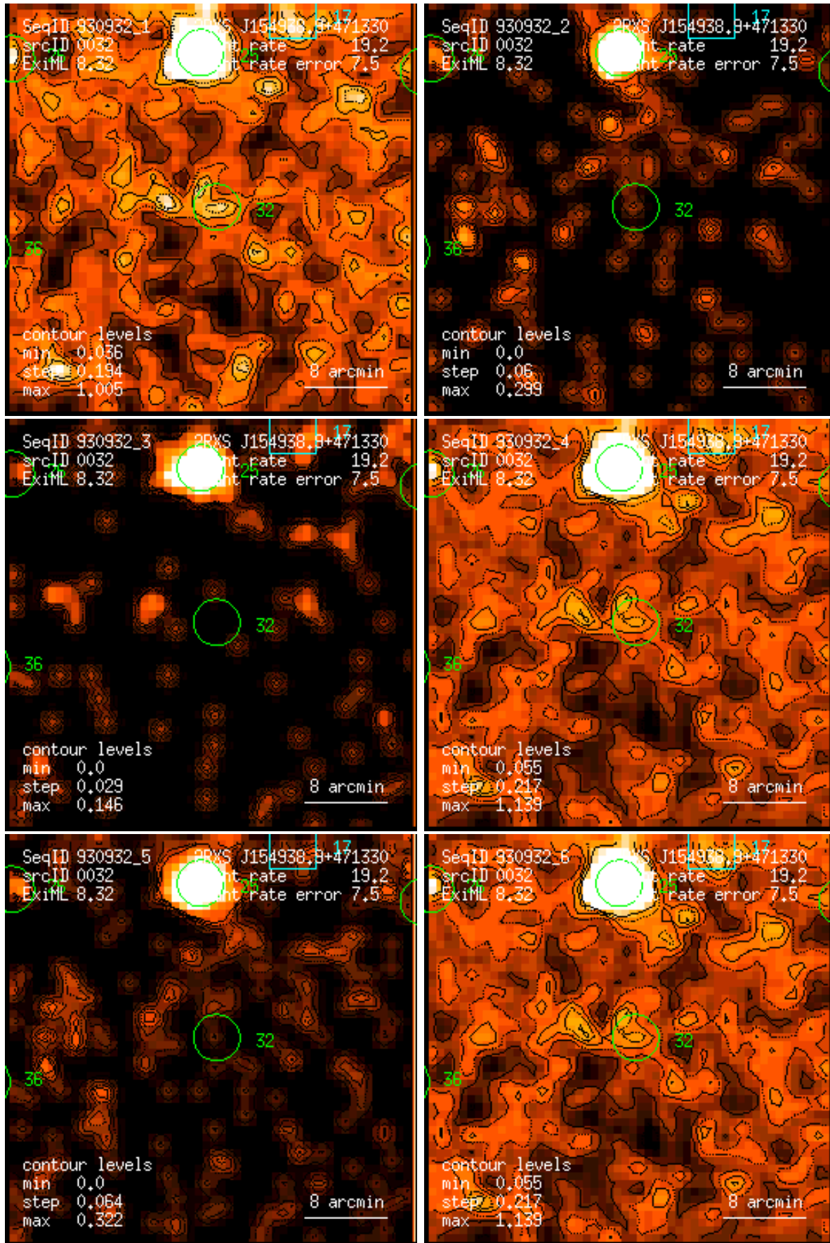
Figure 32: RASS 930932: detection 0032: band rate images, Gaussian filter: (1) PSPC channels 11 – 41, (2) 52 – 90, (3) 91 – 201, (4) 11 – 235, (5) 52 – 201, (6) 11 – 201. Broad band rates in counts/ks. Band rate contour levels in counts/ks/arcmin 2 .
