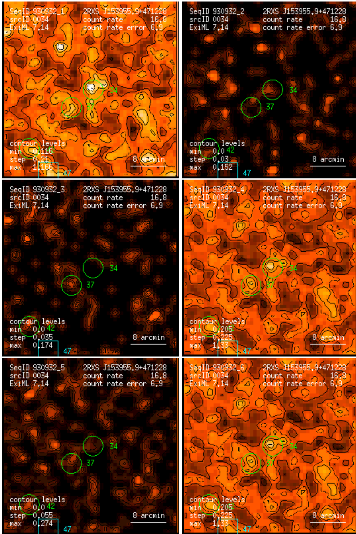
Figure 34: RASS 930932: detection 0034: band rate images, Gaussian filter: (1) PSPC channels 11 – 41, (2) 52 – 90, (3) 91 – 201, (4) 11 – 235, (5) 52 – 201, (6) 11 – 201. Broad band rates in counts/ks. Band rate contour levels in counts/ks/arcmin 2 .
