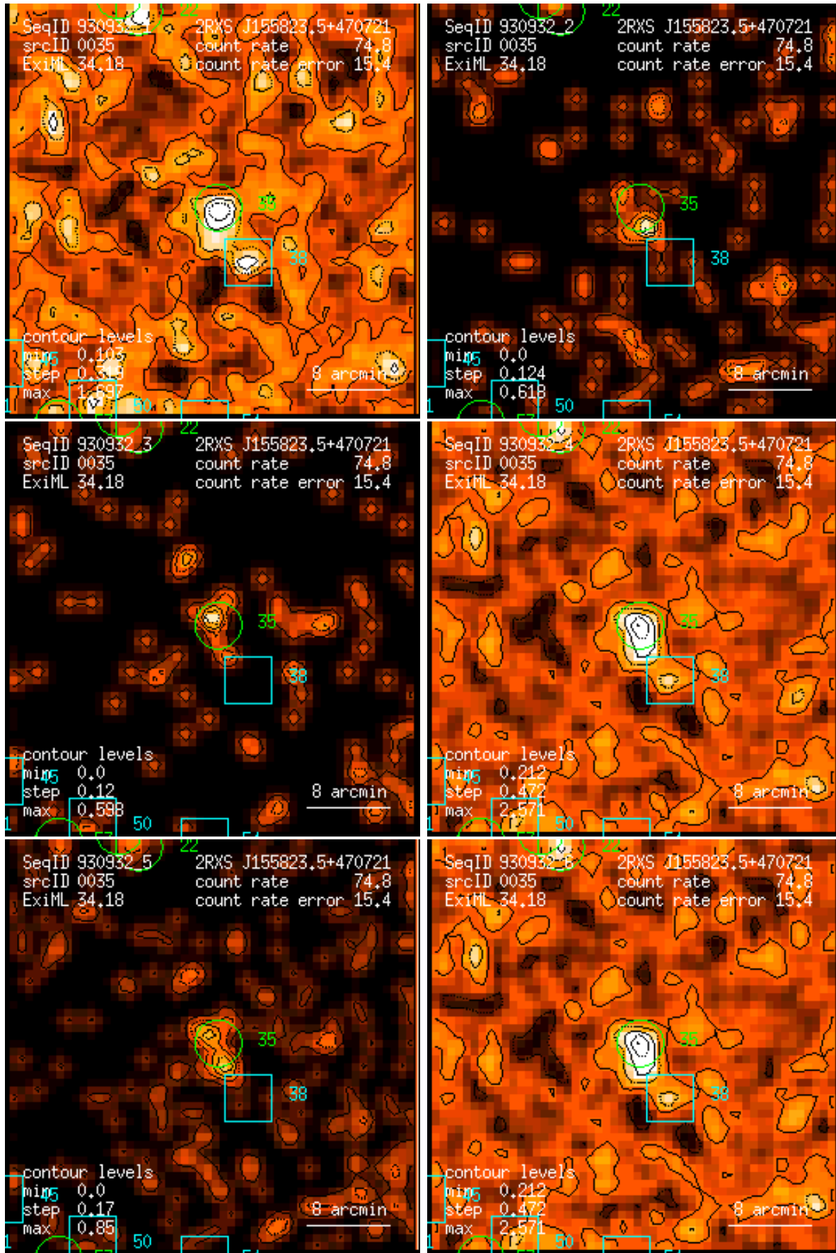
Figure 35: RASS 930932: detection 0035: band rate images, Gaussian filter: (1) PSPC channels 11 – 41, (2) 52 – 90, (3) 91 – 201, (4) 11 – 235, (5) 52 – 201, (6) 11 – 201. Broad band rates in counts/ks. Band rate contour levels in counts/ks/arcmin 2 .
