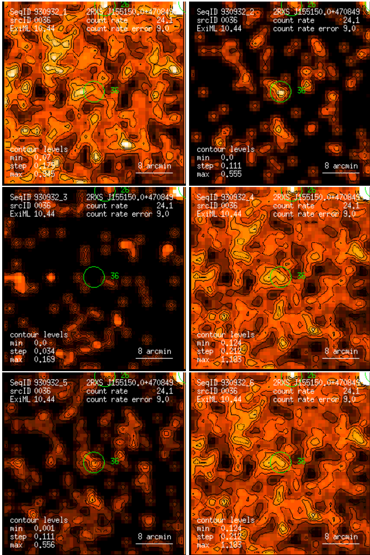
Figure 36: RASS 930932: detection 0036: band rate images, Gaussian filter: (1) PSPC channels 11 – 41, (2) 52 – 90, (3) 91 – 201, (4) 11 – 235, (5) 52 – 201, (6) 11 – 201. Broad band rates in counts/ks. Band rate contour levels in counts/ks/arcmin 2 .
