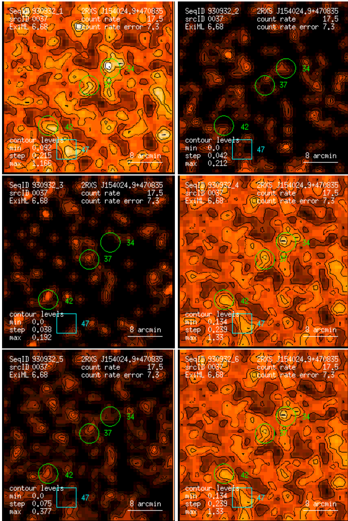
Figure 37: RASS 930932: detection 0037: band rate images, Gaussian filter: (1) PSPC channels 11 – 41, (2) 52 – 90, (3) 91 – 201, (4) 11 – 235, (5) 52 – 201, (6) 11 – 201. Broad band rates in counts/ks. Band rate contour levels in counts/ks/arcmin 2 .
