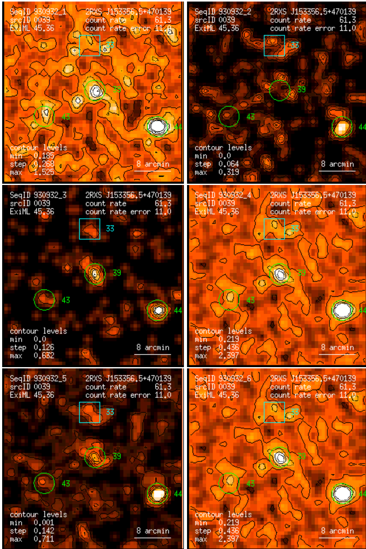
Figure 39: RASS 930932: detection 0039: band rate images, Gaussian filter: (1) PSPC channels 11 – 41, (2) 52 – 90, (3) 91 – 201, (4) 11 – 235, (5) 52 – 201, (6) 11 – 201. Broad band rates in counts/ks. Band rate contour levels in counts/ks/arcmin 2 .
