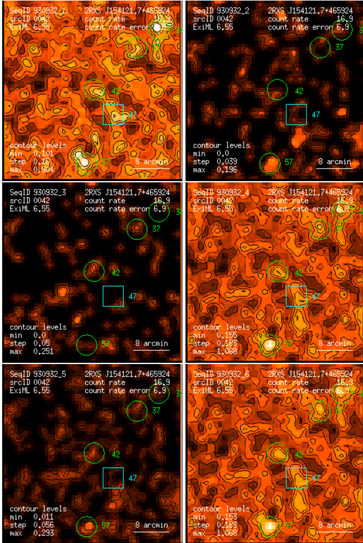
Figure 42: RASS 930932: detection 0042: band rate images, Gaussian filter: (1) PSPC channels 11 – 41, (2) 52 – 90, (3) 91 – 201, (4) 11 – 235, (5) 52 – 201, (6) 11 – 201. Broad band rates in counts/ks. Band rate contour levels in counts/ks/arcmin 2 .
