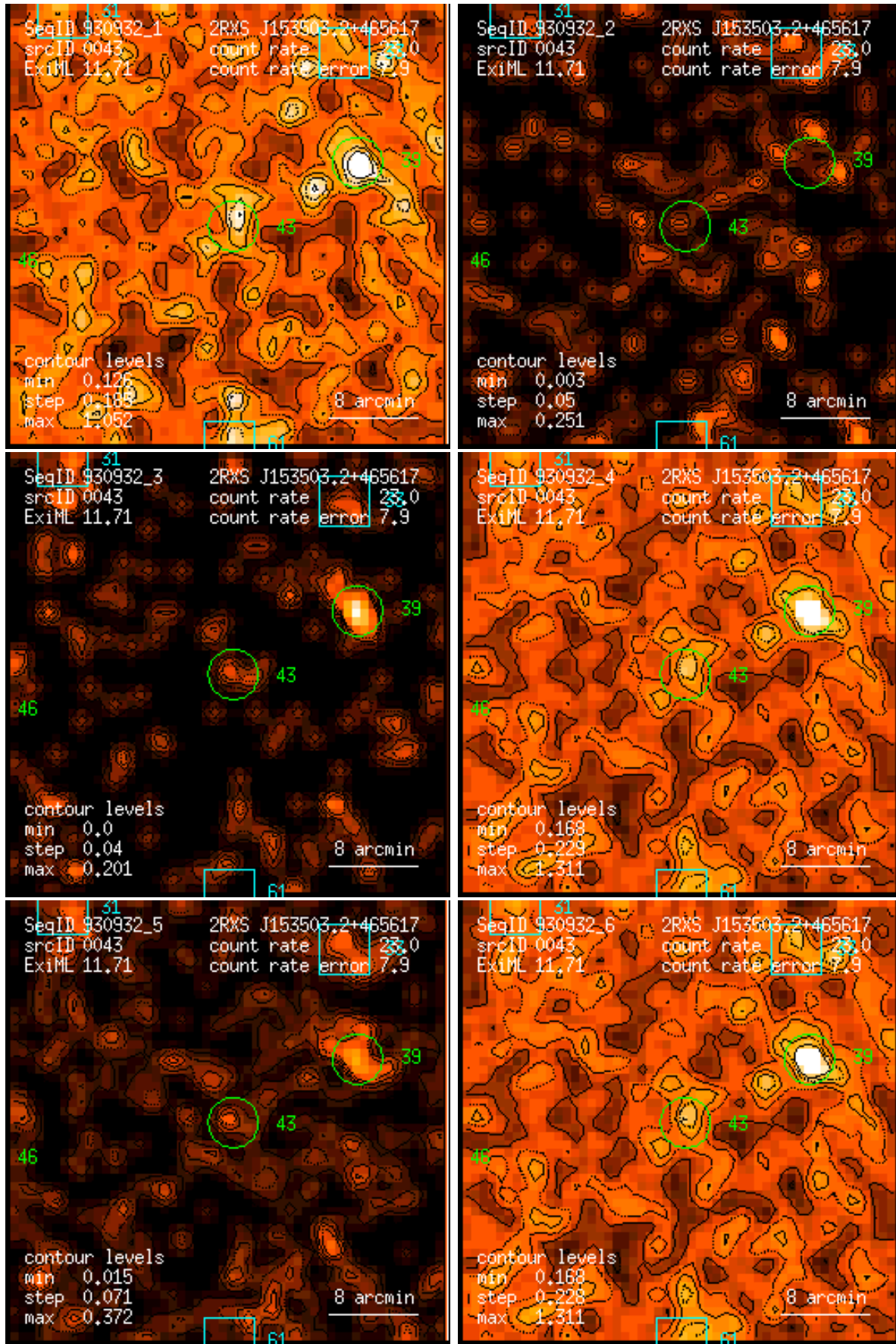
Figure 43: RASS 930932: detection 0043: band rate images, Gaussian filter: (1) PSPC channels 11 – 41, (2) 52 – 90, (3) 91 – 201, (4) 11 – 235, (5) 52 – 201, (6) 11 – 201. Broad band rates in counts/ks. Band rate contour levels in counts/ks/arcmin 2 .
