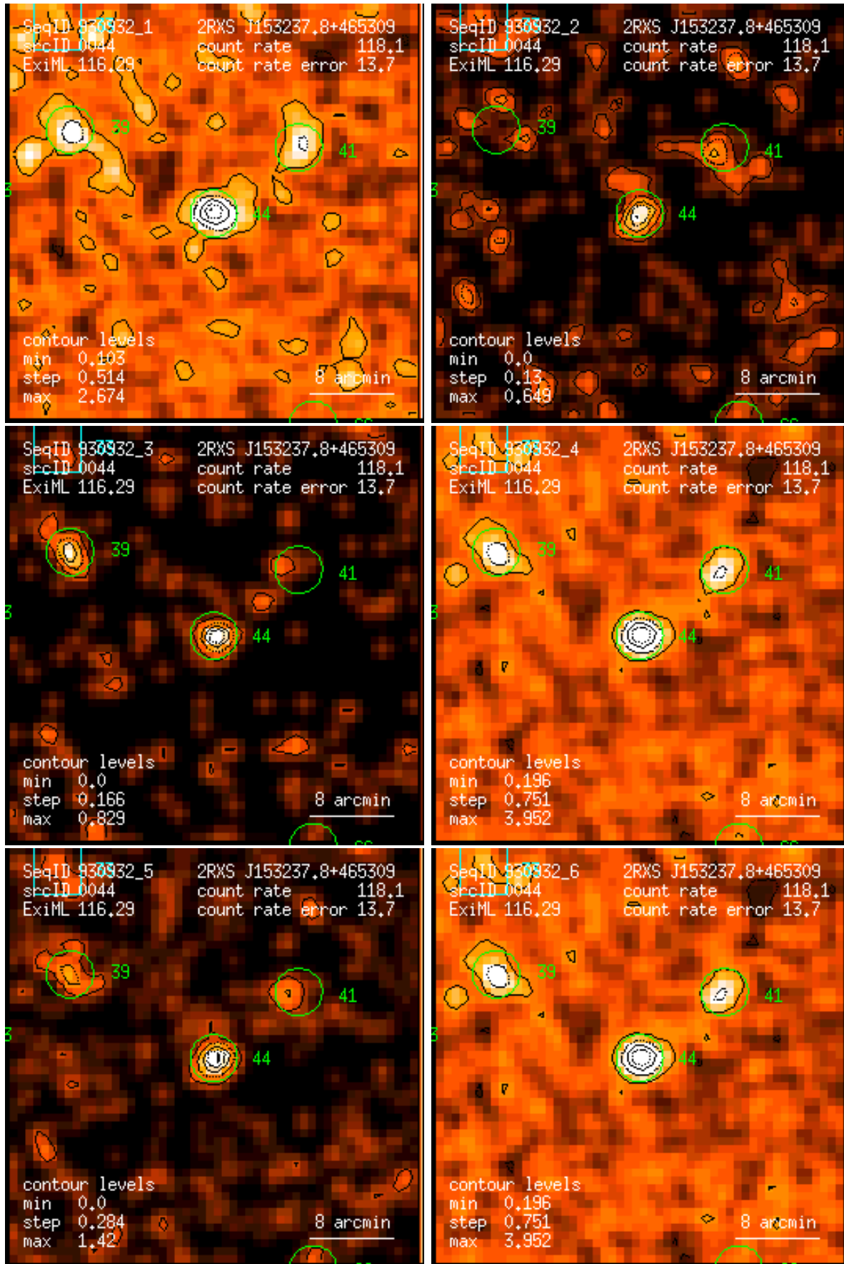
Figure 44: RASS 930932: detection 0044: band rate images, Gaussian filter: (1) PSPC channels 11 – 41, (2) 52 – 90, (3) 91 – 201, (4) 11 – 235, (5) 52 – 201, (6) 11 – 201. Broad band rates in counts/ks. Band rate contour levels in counts/ks/arcmin 2 .
