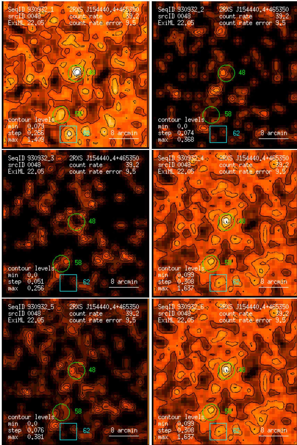
Figure 48: RASS 930932: detection 0048: band rate images, Gaussian filter: (1) PSPC channels 11 – 41, (2) 52 – 90, (3) 91 – 201, (4) 11 – 235, (5) 52 – 201, (6) 11 – 201. Broad band rates in counts/ks. Band rate contour levels in counts/ks/arcmin 2 .
