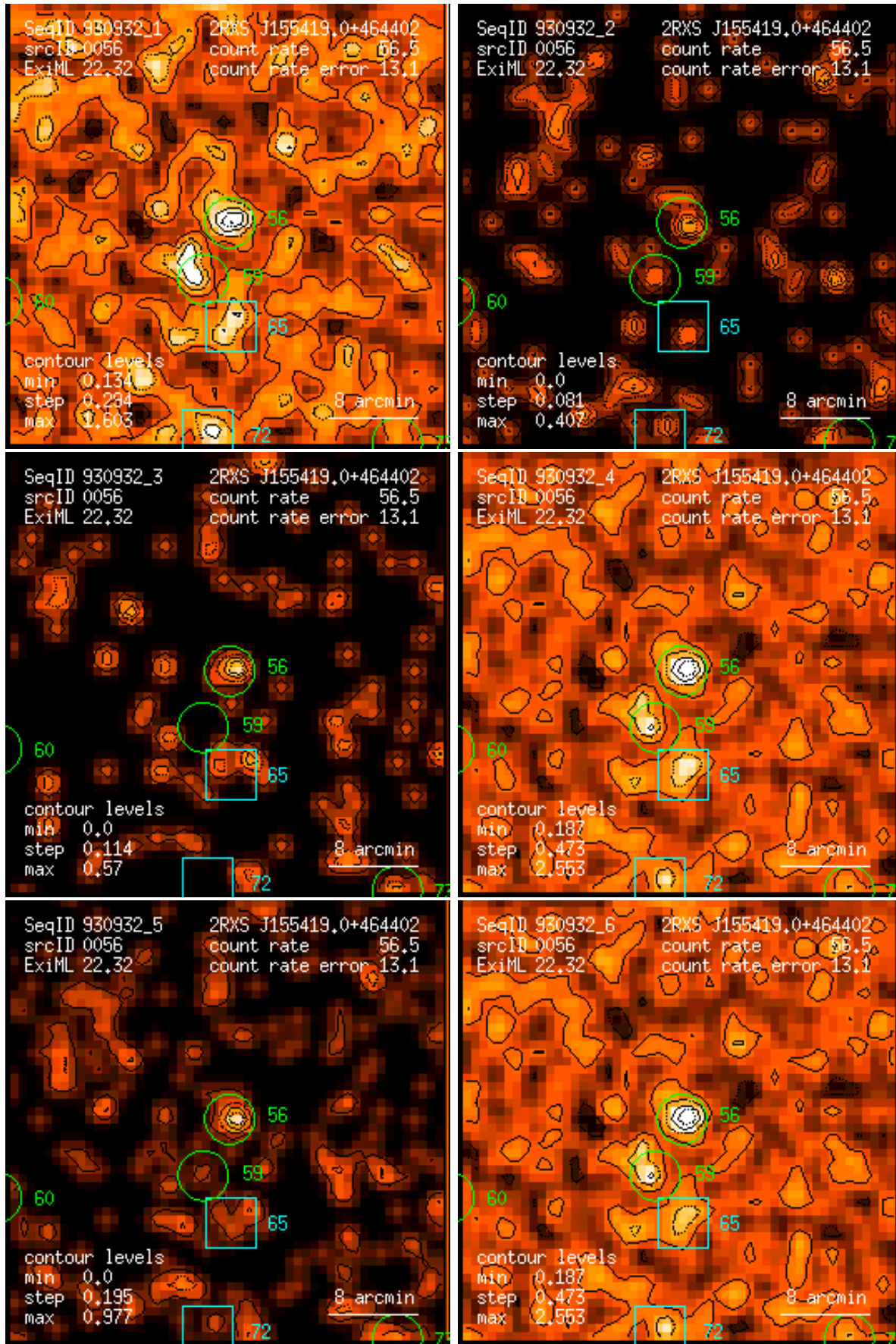
Figure 56: RASS 930932: detection 0056: band rate images, Gaussian filter: (1) PSPC channels 11 – 41, (2) 52 – 90, (3) 91 – 201, (4) 11 – 235, (5) 52 – 201, (6) 11 – 201. Broad band rates in counts/ks. Band rate contour levels in counts/ks/arcmin 2 .
