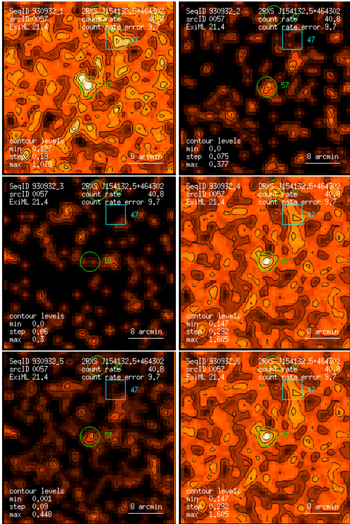
Figure 57: RASS 930932: detection 0057: band rate images, Gaussian filter: (1) PSPC channels 11 – 41, (2) 52 – 90, (3) 91 – 201, (4) 11 – 235, (5) 52 – 201, (6) 11 – 201. Broad band rates in counts/ks. Band rate contour levels in counts/ks/arcmin 2 .
