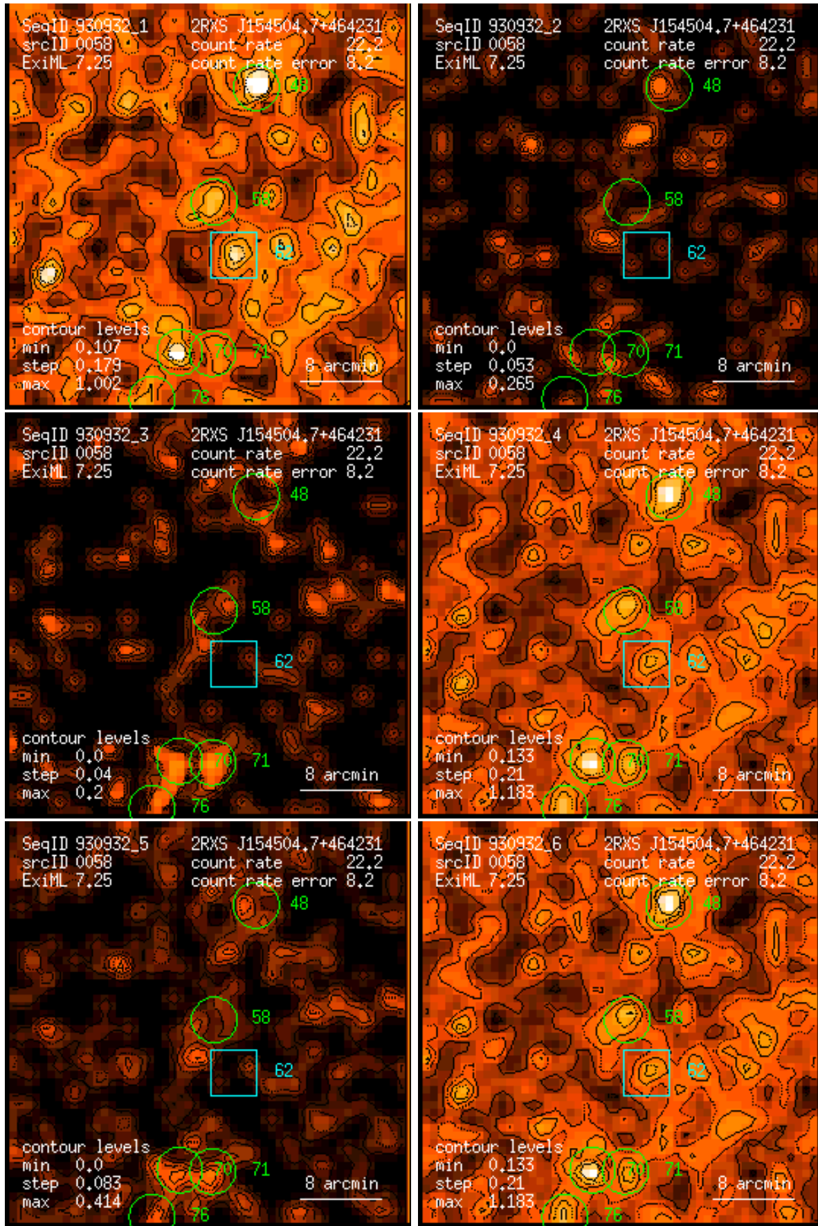
Figure 58: RASS 930932: detection 0058: band rate images, Gaussian filter: (1) PSPC channels 11 – 41, (2) 52 – 90, (3) 91 – 201, (4) 11 – 235, (5) 52 – 201, (6) 11 – 201. Broad band rates in counts/ks. Band rate contour levels in counts/ks/arcmin 2 .
