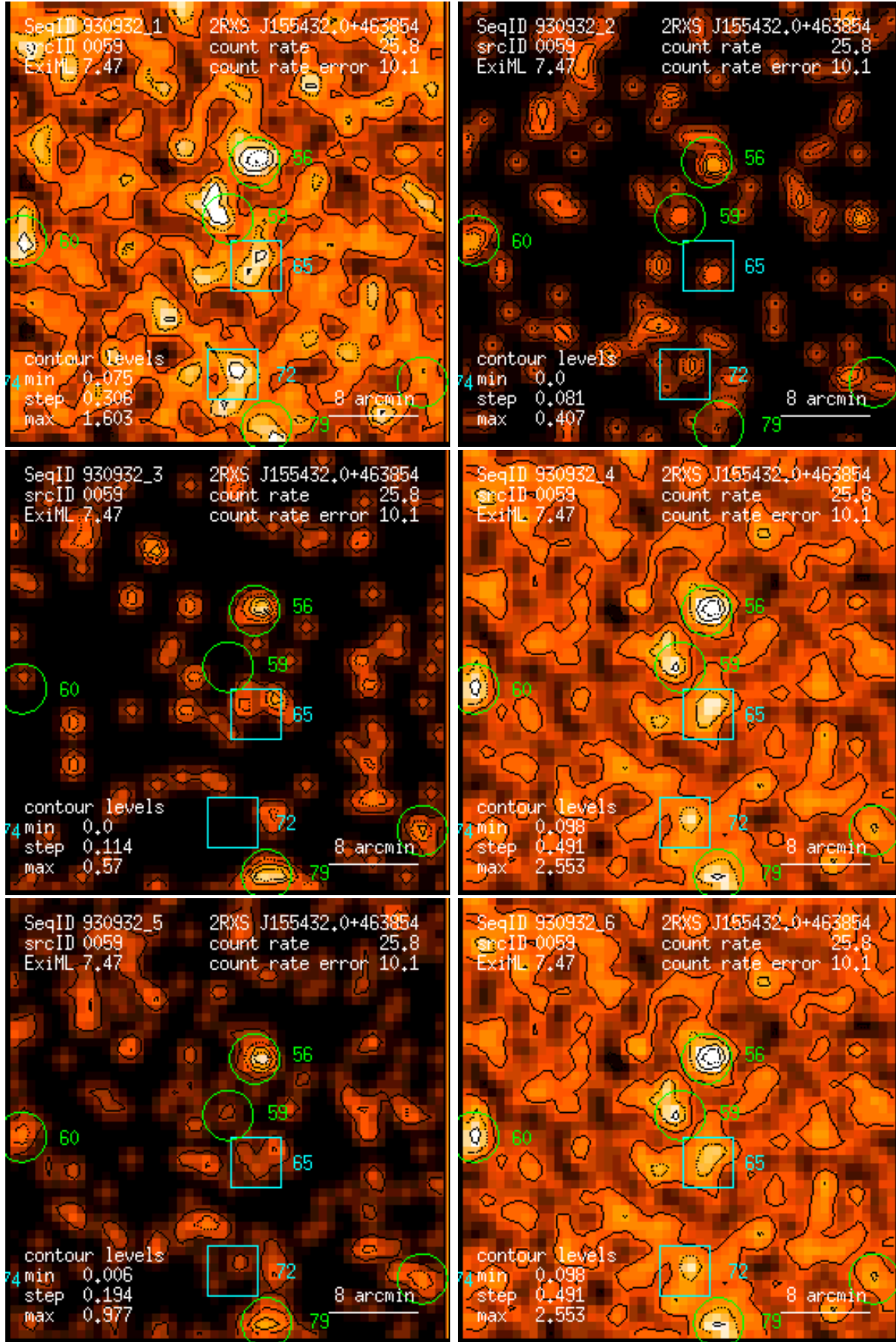
Figure 59: RASS 930932: detection 0059: band rate images, Gaussian filter: (1) PSPC channels 11 – 41, (2) 52 – 90, (3) 91 – 201, (4) 11 – 235, (5) 52 – 201, (6) 11 – 201. Broad band rates in counts/ks. Band rate contour levels in counts/ks/arcmin 2 .
