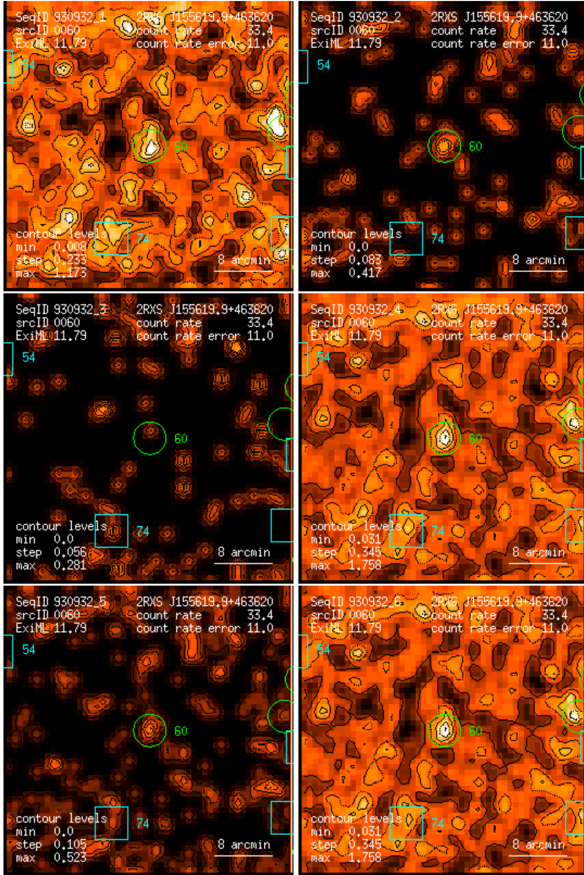
Figure 60: RASS 930932: detection 0060: band rate images, Gaussian filter: (1) PSPC channels 11 – 41, (2) 52 – 90, (3) 91 – 201, (4) 11 – 235, (5) 52 – 201, (6) 11 – 201. Broad band rates in counts/ks. Band rate contour levels in counts/ks/arcmin 2 .
