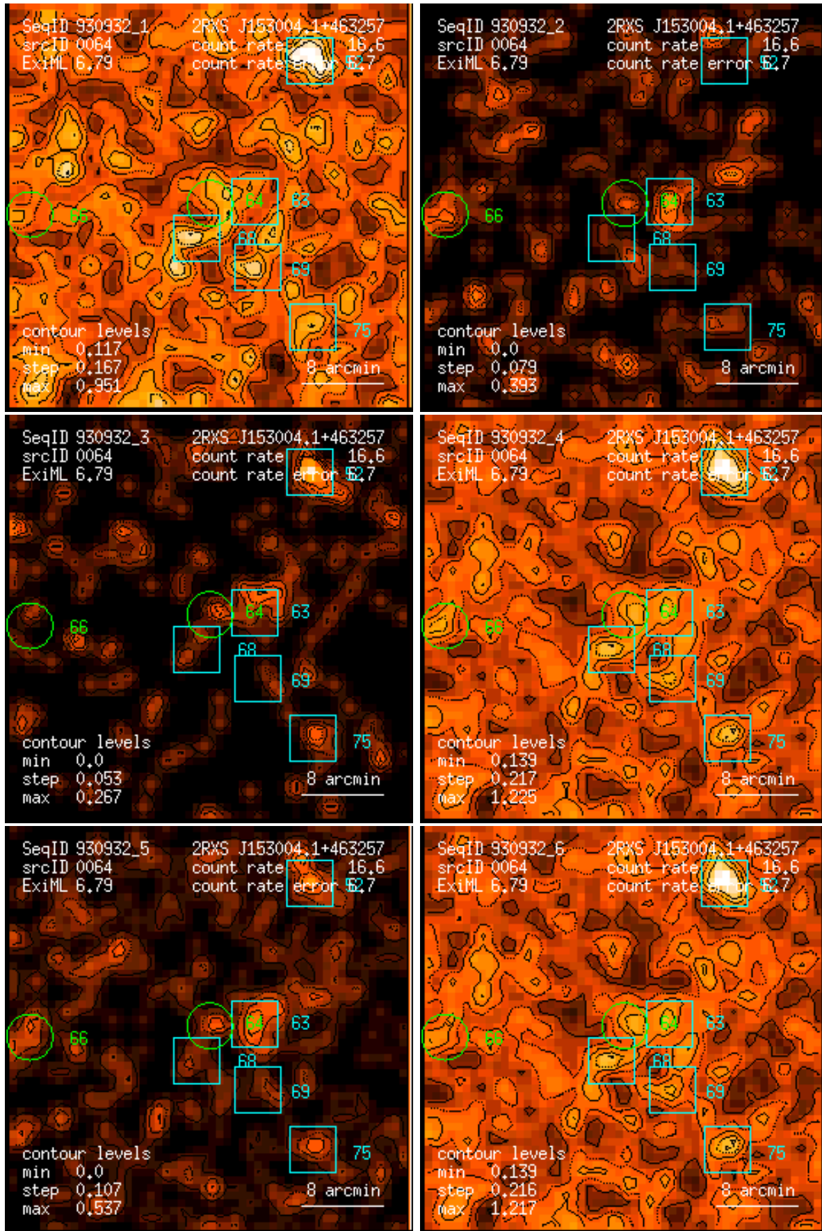
Figure 64: RASS 930932: detection 0064: band rate images, Gaussian filter: (1) PSPC channels 11 – 41, (2) 52 – 90, (3) 91 – 201, (4) 11 – 235, (5) 52 – 201, (6) 11 – 201. Broad band rates in counts/ks. Band rate contour levels in counts/ks/arcmin 2 .
