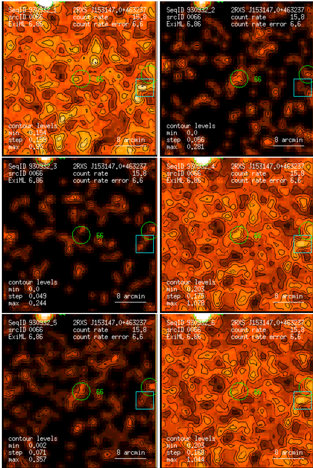
Figure 66: RASS 930932: detection 0066: band rate images, Gaussian filter: (1) PSPC channels 11 – 41, (2) 52 – 90, (3) 91 – 201, (4) 11 – 235, (5) 52 – 201, (6) 11 – 201. Broad band rates in counts/ks. Band rate contour levels in counts/ks/arcmin 2 .
