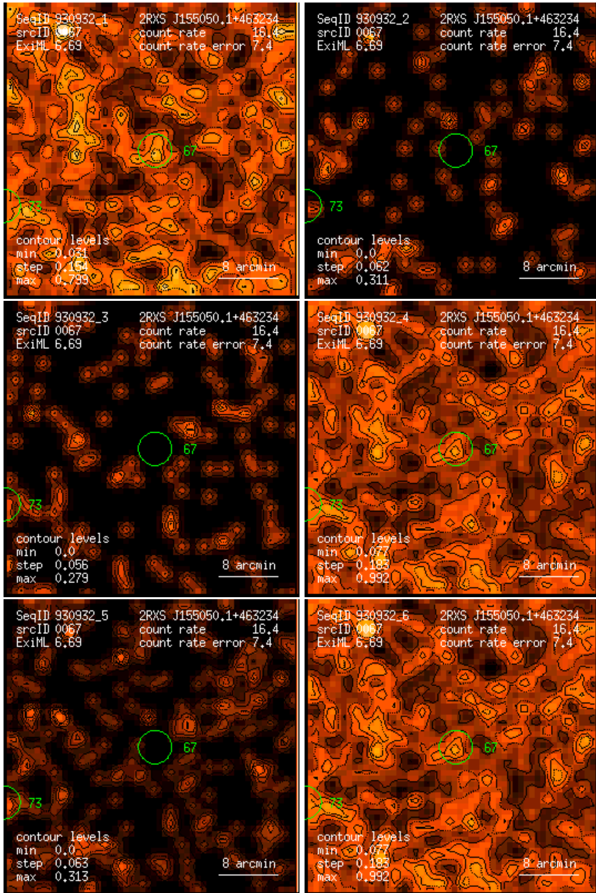
Figure 67: RASS 930932: detection 0067: band rate images, Gaussian filter: (1) PSPC channels 11 – 41, (2) 52 – 90, (3) 91 – 201, (4) 11 – 235, (5) 52 – 201, (6) 11 – 201. Broad band rates in counts/ks. Band rate contour levels in counts/ks/arcmin 2 .
