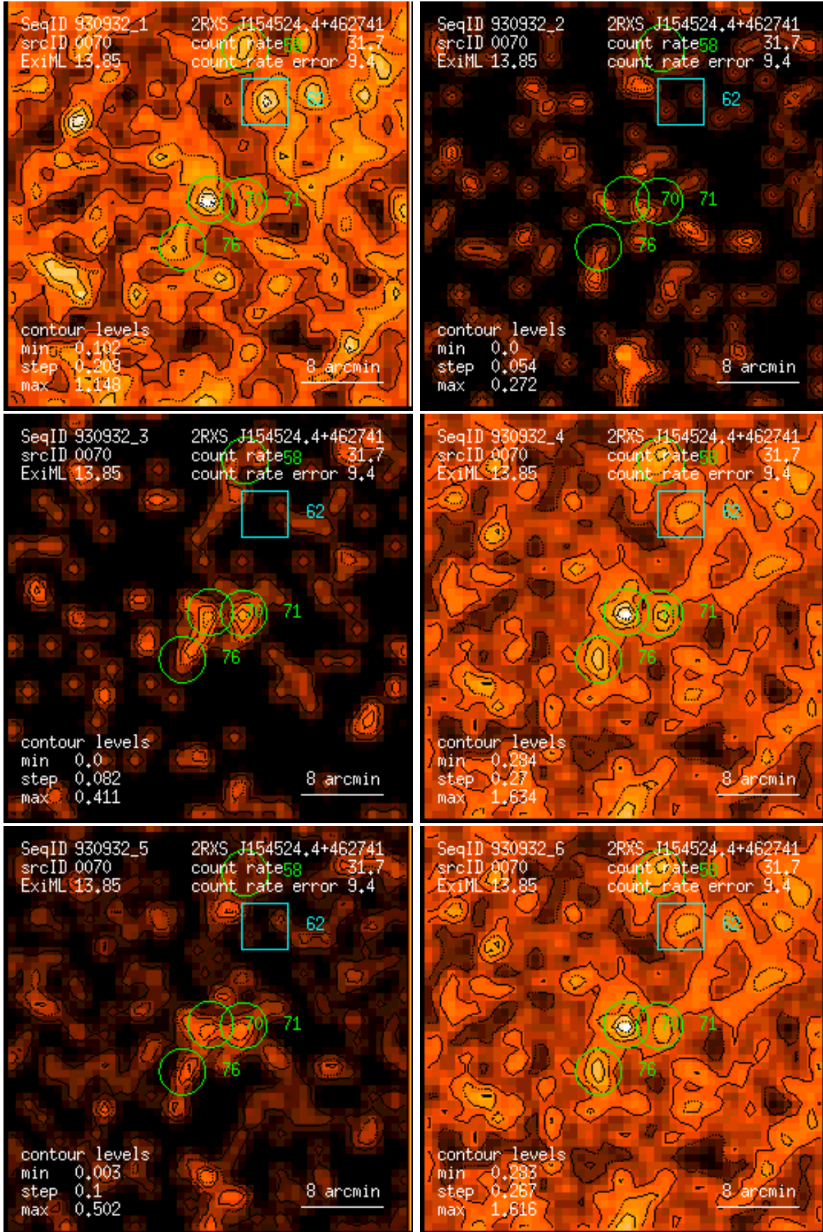
Figure 70: RASS 930932: detection 0070: band rate images, Gaussian filter: (1) PSPC channels 11 – 41, (2) 52 – 90, (3) 91 – 201, (4) 11 – 235, (5) 52 – 201, (6) 11 – 201. Broad band rates in counts/ks. Band rate contour levels in counts/ks/arcmin 2 .
