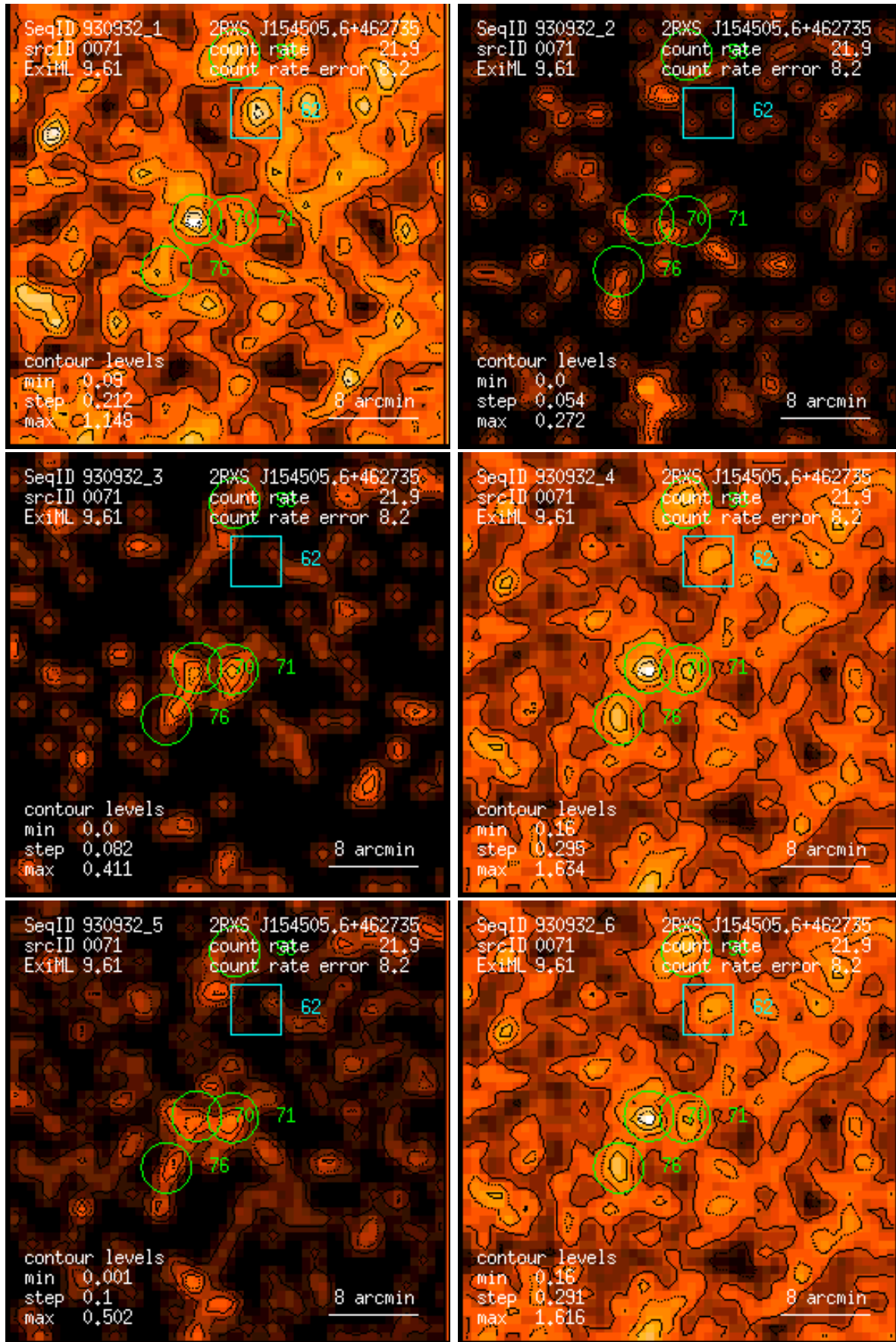
Figure 71: RASS 930932: detection 0071: band rate images, Gaussian filter: (1) PSPC channels 11 – 41, (2) 52 – 90, (3) 91 – 201, (4) 11 – 235, (5) 52 – 201, (6) 11 – 201. Broad band rates in counts/ks. Band rate contour levels in counts/ks/arcmin 2 .
