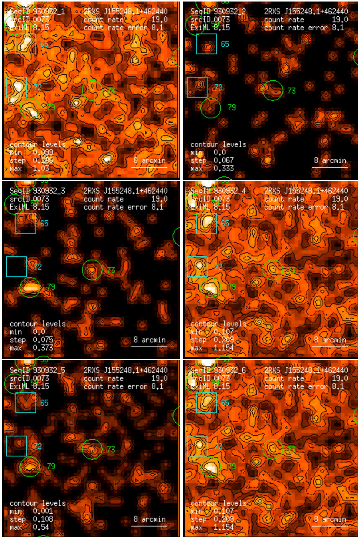
Figure 73: RASS 930932: detection 0073: band rate images, Gaussian filter: (1) PSPC channels 11 – 41, (2) 52 – 90, (3) 91 – 201, (4) 11 – 235, (5) 52 – 201, (6) 11 – 201. Broad band rates in counts/ks. Band rate contour levels in counts/ks/arcmin 2 .
