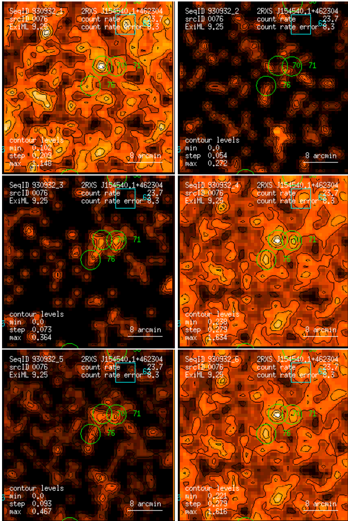
Figure 76: RASS 930932: detection 0076: band rate images, Gaussian filter: (1) PSPC channels 11 – 41, (2) 52 – 90, (3) 91 – 201, (4) 11 – 235, (5) 52 – 201, (6) 11 – 201. Broad band rates in counts/ks. Band rate contour levels in counts/ks/arcmin 2 .
