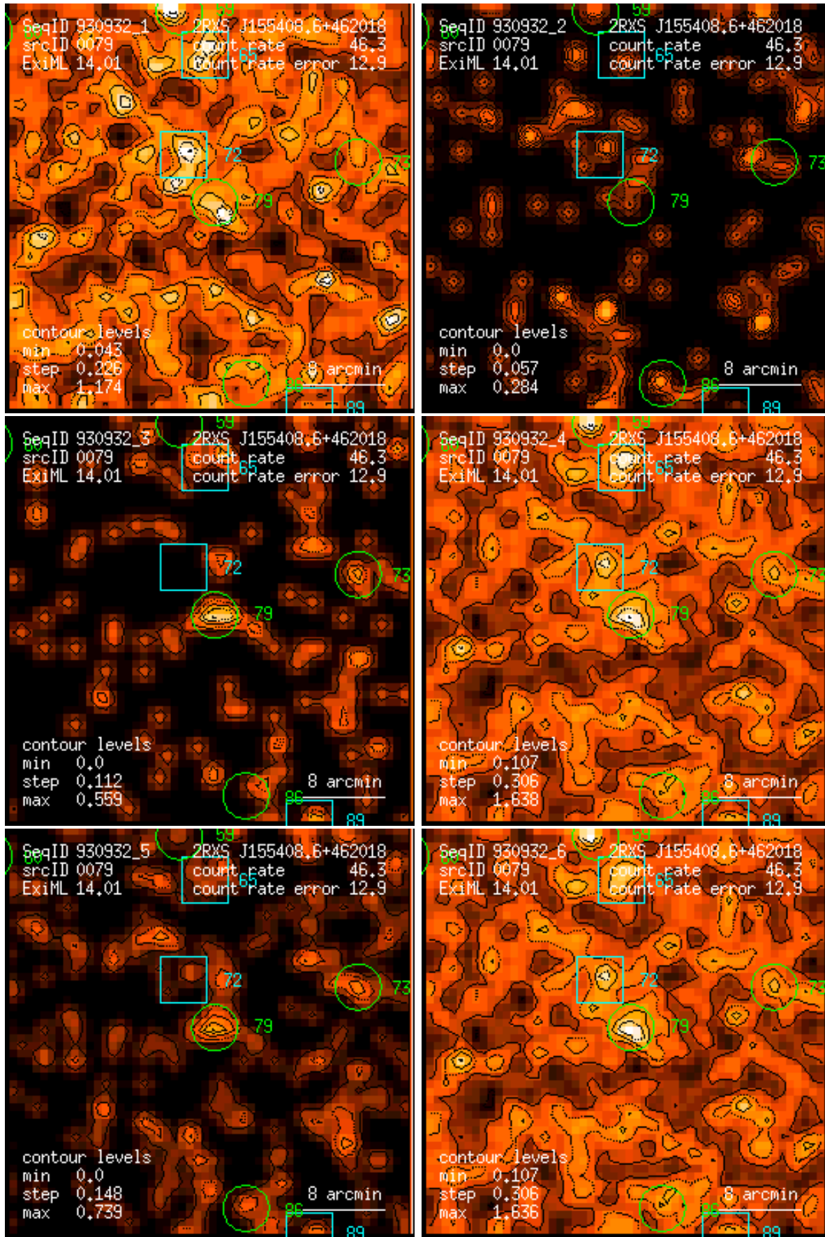
Figure 79: RASS 930932: detection 0079: band rate images, Gaussian filter: (1) PSPC channels 11 – 41, (2) 52 – 90, (3) 91 – 201, (4) 11 – 235, (5) 52 – 201, (6) 11 – 201. Broad band rates in counts/ks. Band rate contour levels in counts/ks/arcmin 2 .
