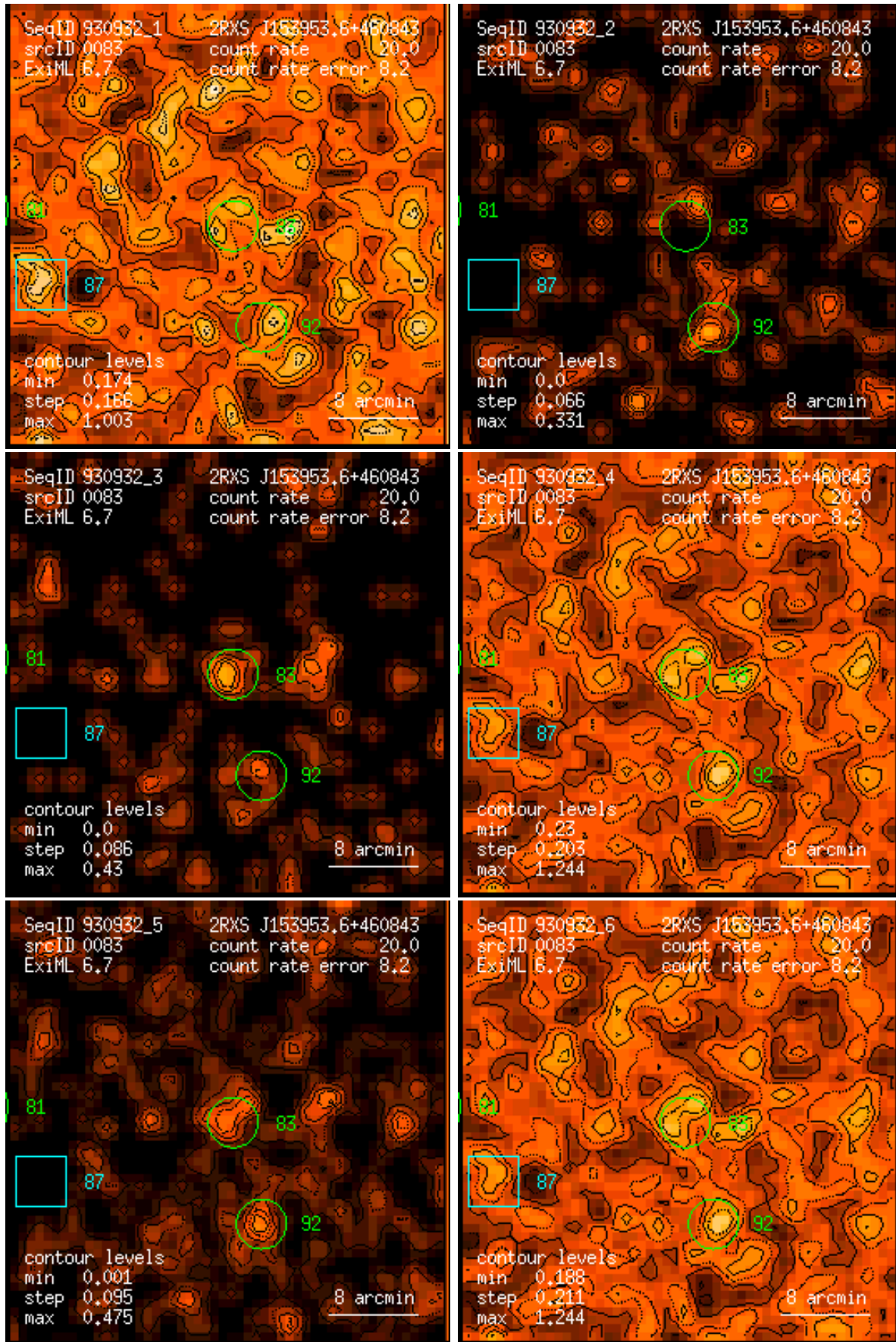
Figure 83: RASS 930932: detection 0083: band rate images, Gaussian filter: (1) PSPC channels 11 – 41, (2) 52 – 90, (3) 91 – 201, (4) 11 – 235, (5) 52 – 201, (6) 11 – 201. Broad band rates in counts/ks. Band rate contour levels in counts/ks/arcmin 2 .
