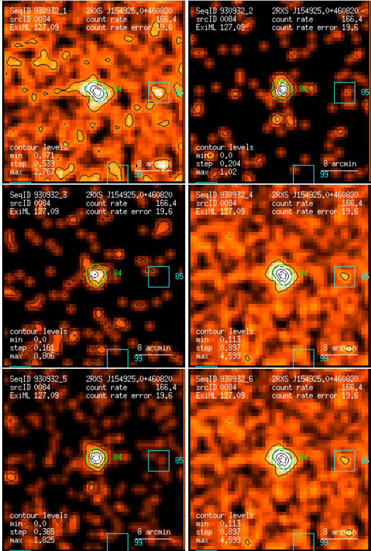
Figure 84: RASS 930932: detection 0084: band rate images, Gaussian filter: (1) PSPC channels 11 – 41, (2) 52 – 90, (3) 91 – 201, (4) 11 – 235, (5) 52 – 201, (6) 11 – 201. Broad band rates in counts/ks. Band rate contour levels in counts/ks/arcmin 2 .
