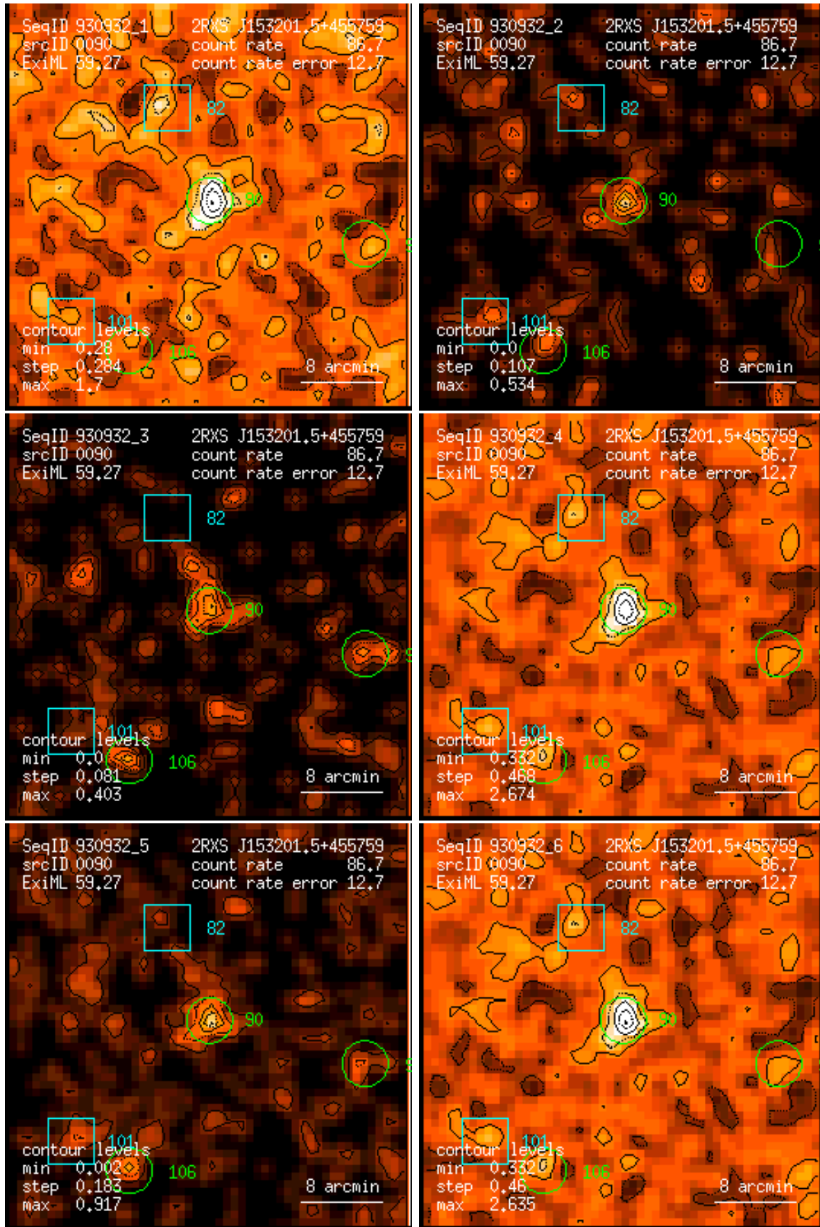
Figure 90: RASS 930932: detection 0090: band rate images, Gaussian filter: (1) PSPC channels 11 – 41, (2) 52 – 90, (3) 91 – 201, (4) 11 – 235, (5) 52 – 201, (6) 11 – 201. Broad band rates in counts/ks. Band rate contour levels in counts/ks/arcmin 2 .
