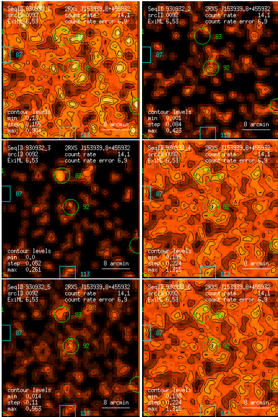
Figure 92: RASS 930932: detection 0092: band rate images, Gaussian filter: (1) PSPC channels 11 – 41, (2) 52 – 90, (3) 91 – 201, (4) 11 – 235, (5) 52 – 201, (6) 11 – 201. Broad band rates in counts/ks. Band rate contour levels in counts/ks/arcmin 2 .
