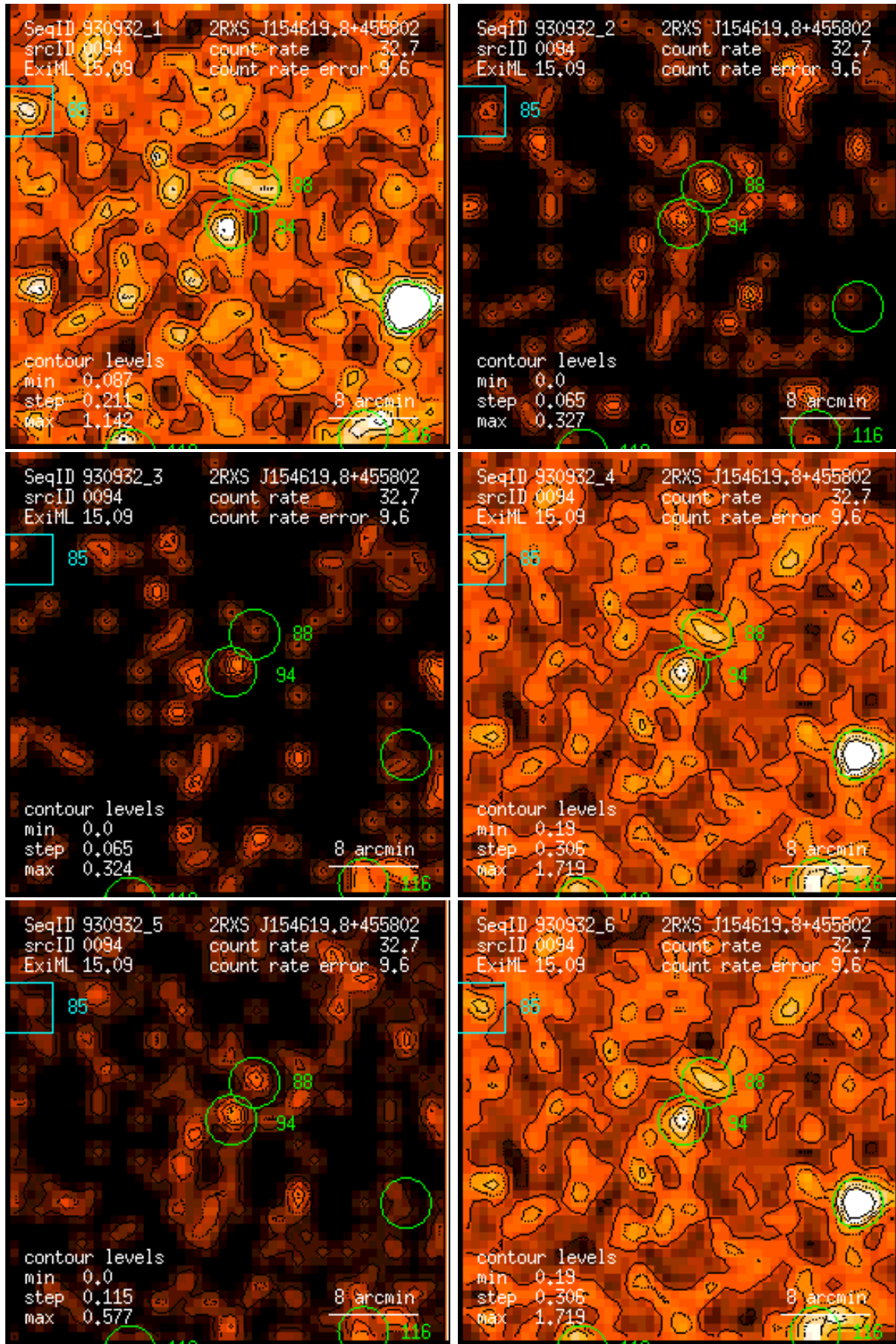
Figure 94: RASS 930932: detection 0094: band rate images, Gaussian filter: (1) PSPC channels 11 – 41, (2) 52 – 90, (3) 91 – 201, (4) 11 – 235, (5) 52 – 201, (6) 11 – 201. Broad band rates in counts/ks. Band rate contour levels in counts/ks/arcmin 2 .
