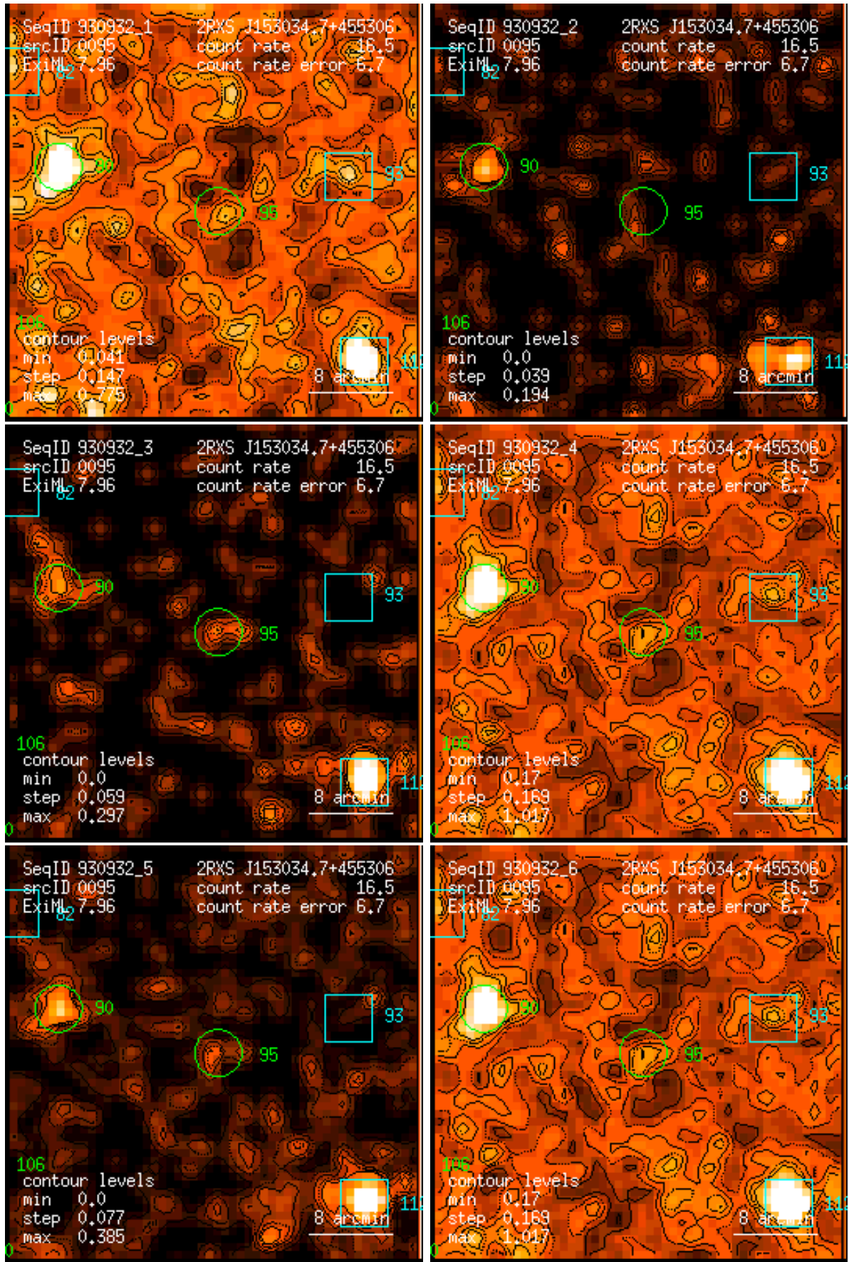
Figure 95: RASS 930932: detection 0095: band rate images, Gaussian filter: (1) PSPC channels 11 – 41, (2) 52 – 90, (3) 91 – 201, (4) 11 – 235, (5) 52 – 201, (6) 11 – 201. Broad band rates in counts/ks. Band rate contour levels in counts/ks/arcmin 2 .
