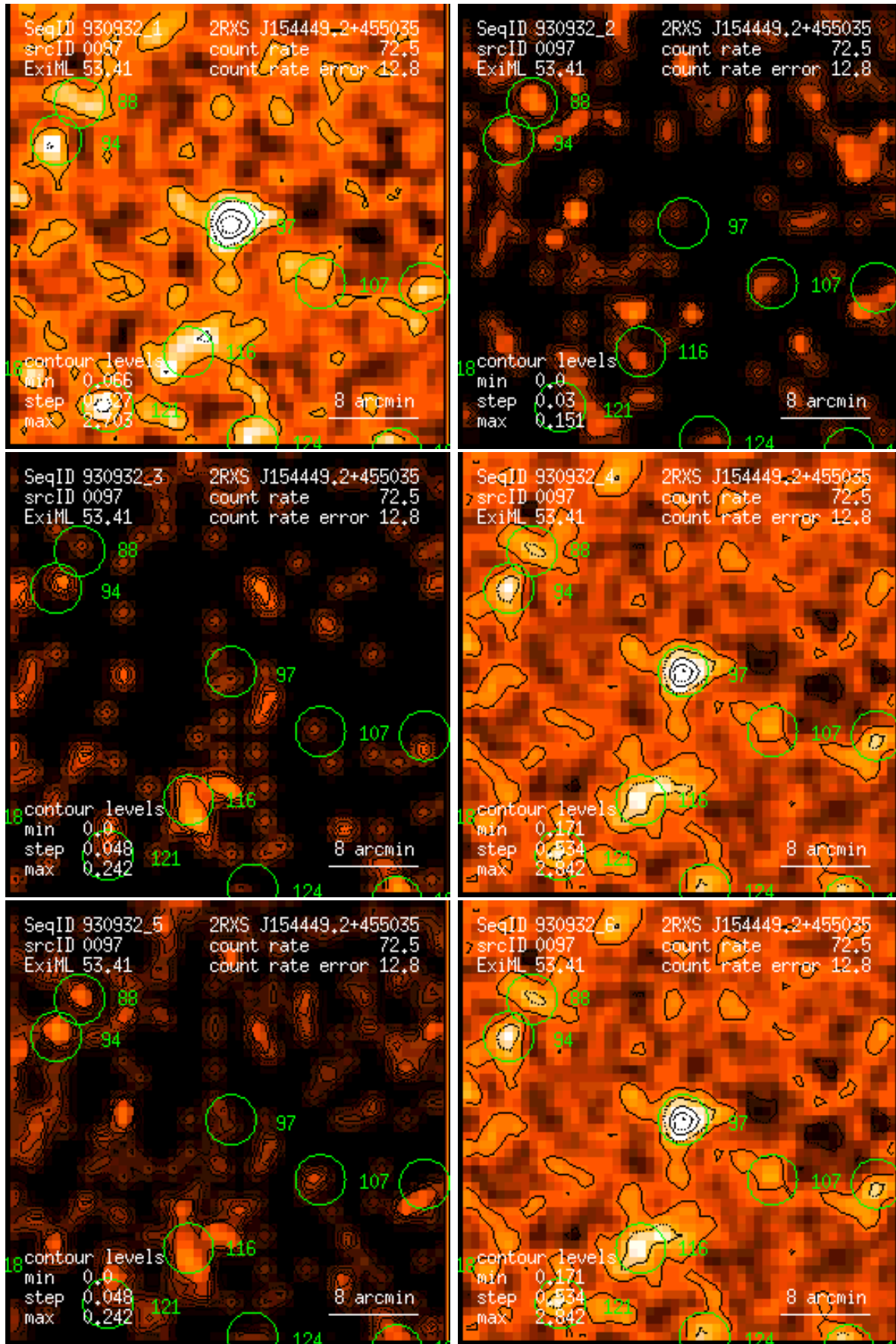
Figure 97: RASS 930932: detection 0097: band rate images, Gaussian filter: (1) PSPC channels 11 – 41, (2) 52 – 90, (3) 91 – 201, (4) 11 – 235, (5) 52 – 201, (6) 11 – 201. Broad band rates in counts/ks. Band rate contour levels in counts/ks/arcmin 2 .
