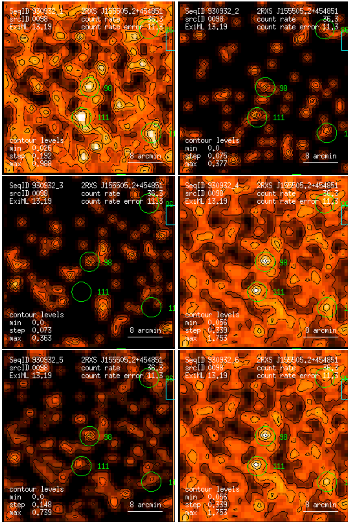
Figure 98: RASS 930932: detection 0098: band rate images, Gaussian filter: (1) PSPC channels 11 – 41, (2) 52 – 90, (3) 91 – 201, (4) 11 – 235, (5) 52 – 201, (6) 11 – 201. Broad band rates in counts/ks. Band rate contour levels in counts/ks/arcmin 2 .
