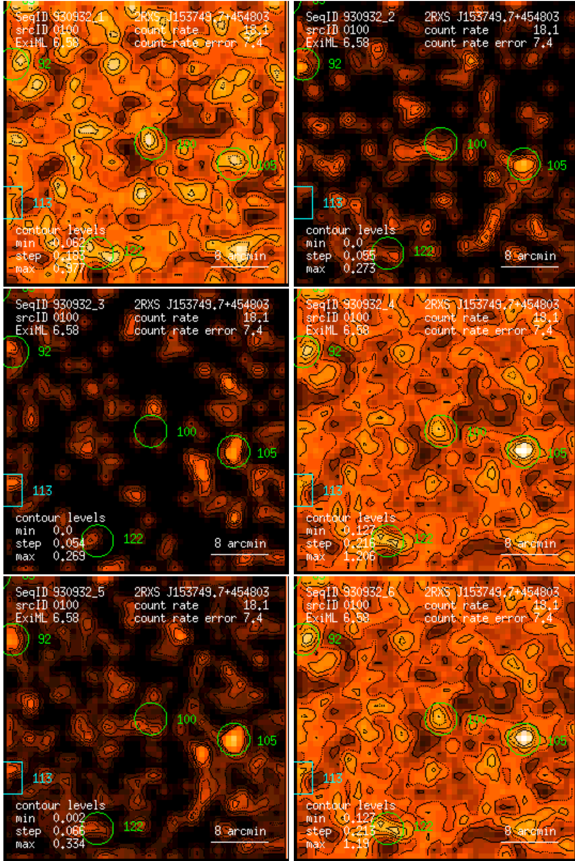
Figure 100: RASS 930932: detection 0100: band rate images, Gaussian filter: (1) PSPC channels 11 – 41, (2) 52 – 90, (3) 91 – 201, (4) 11 – 235, (5) 52 – 201, (6) 11 – 201. Broad band rates in counts/ks. Band rate contour levels in counts/ks/arcmin 2 .
