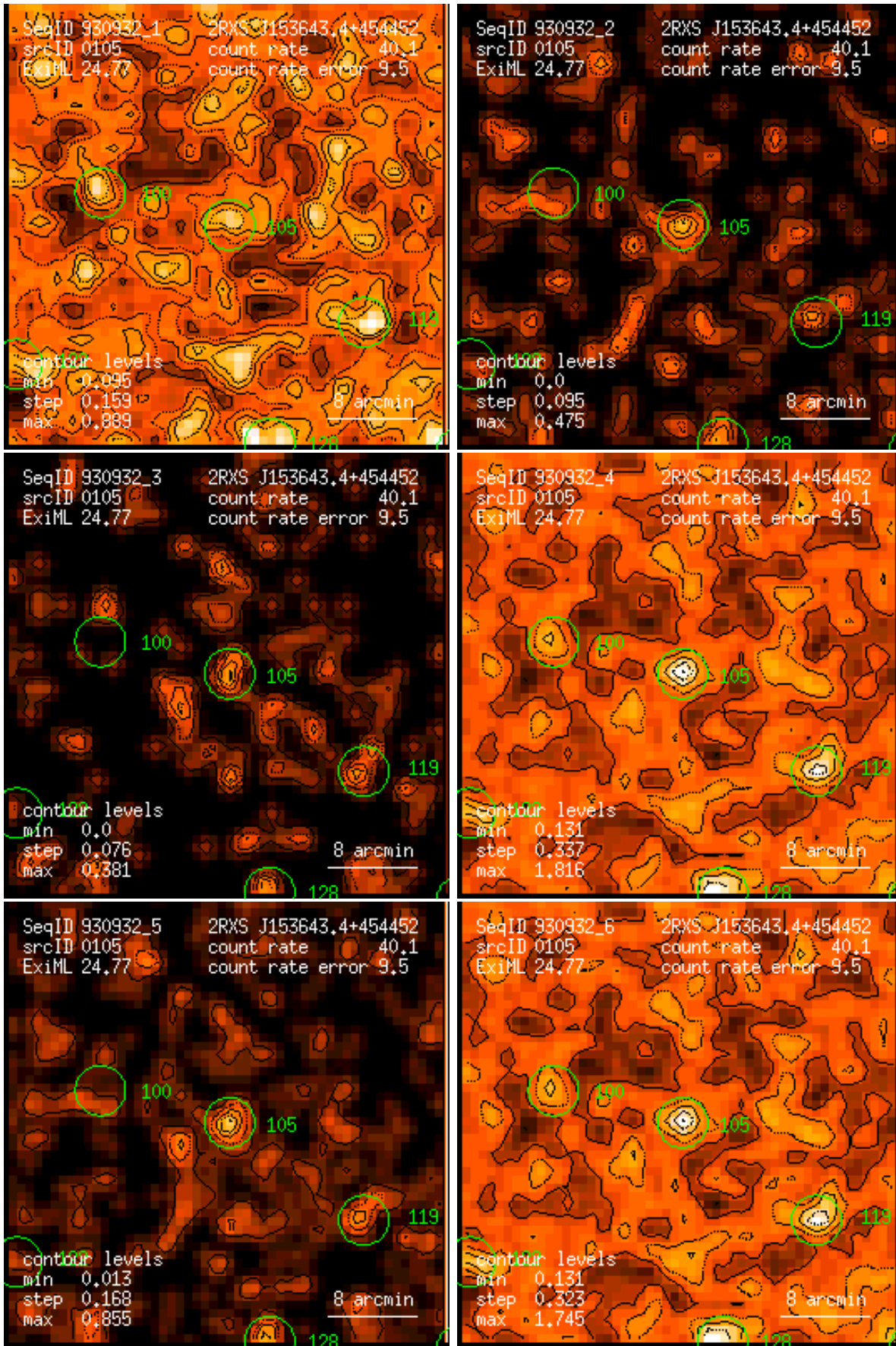
Figure 105: RASS 930932: detection 0105: band rate images, Gaussian filter: (1) PSPC channels 11 – 41, (2) 52 – 90, (3) 91 – 201, (4) 11 – 235, (5) 52 – 201, (6) 11 – 201. Broad band rates in counts/ks. Band rate contour levels in counts/ks/arcmin 2 .
