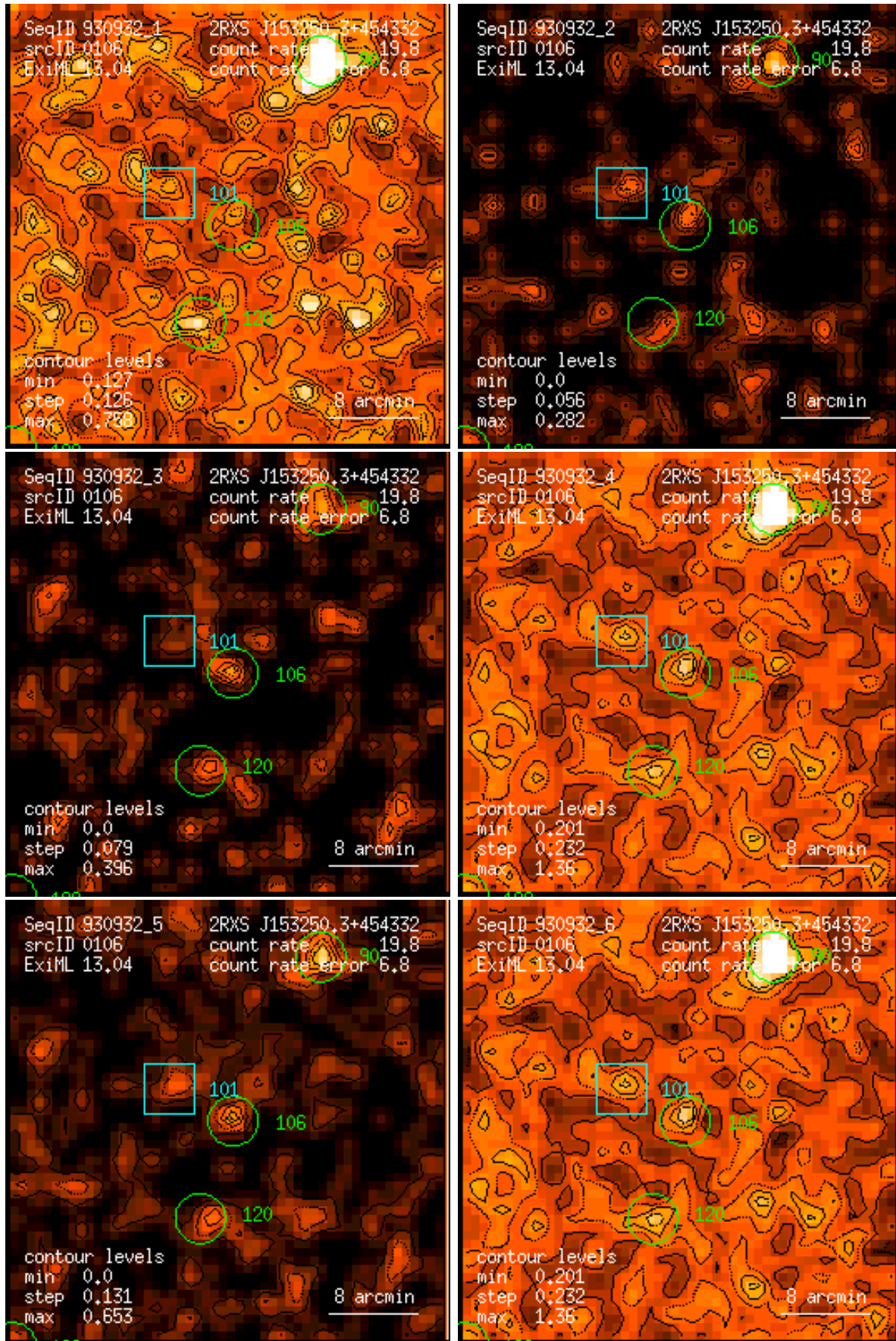
Figure 106: RASS 930932: detection 0106: band rate images, Gaussian filter: (1) PSPC channels 11 – 41, (2) 52 – 90, (3) 91 – 201, (4) 11 – 235, (5) 52 – 201, (6) 11 – 201. Broad band rates in counts/ks. Band rate contour levels in counts/ks/arcmin 2 .
