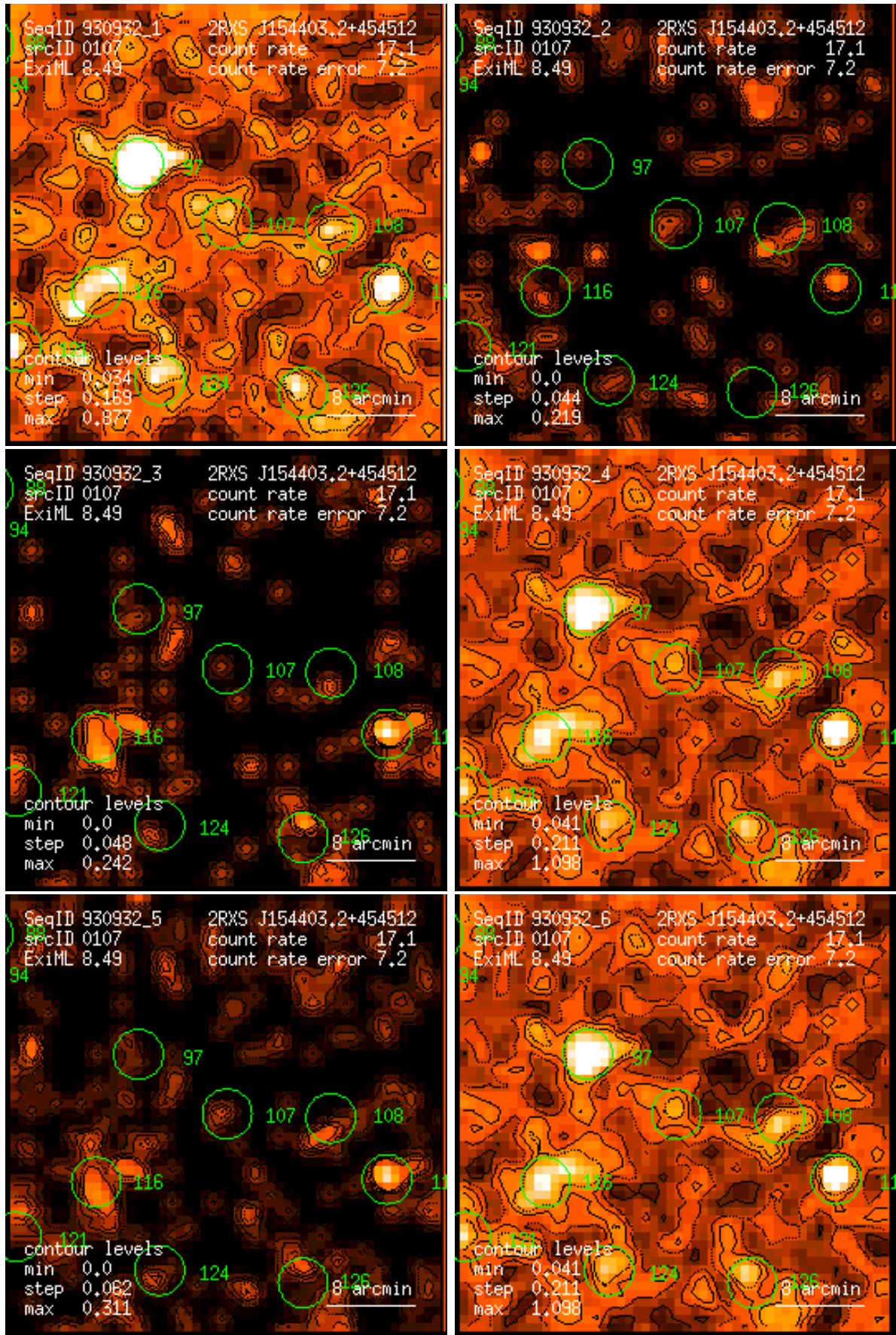
Figure 107: RASS 930932: detection 0107: band rate images, Gaussian filter: (1) PSPC channels 11 – 41, (2) 52 – 90, (3) 91 – 201, (4) 11 – 235, (5) 52 – 201, (6) 11 – 201. Broad band rates in counts/ks. Band rate contour levels in counts/ks/arcmin 2 .
