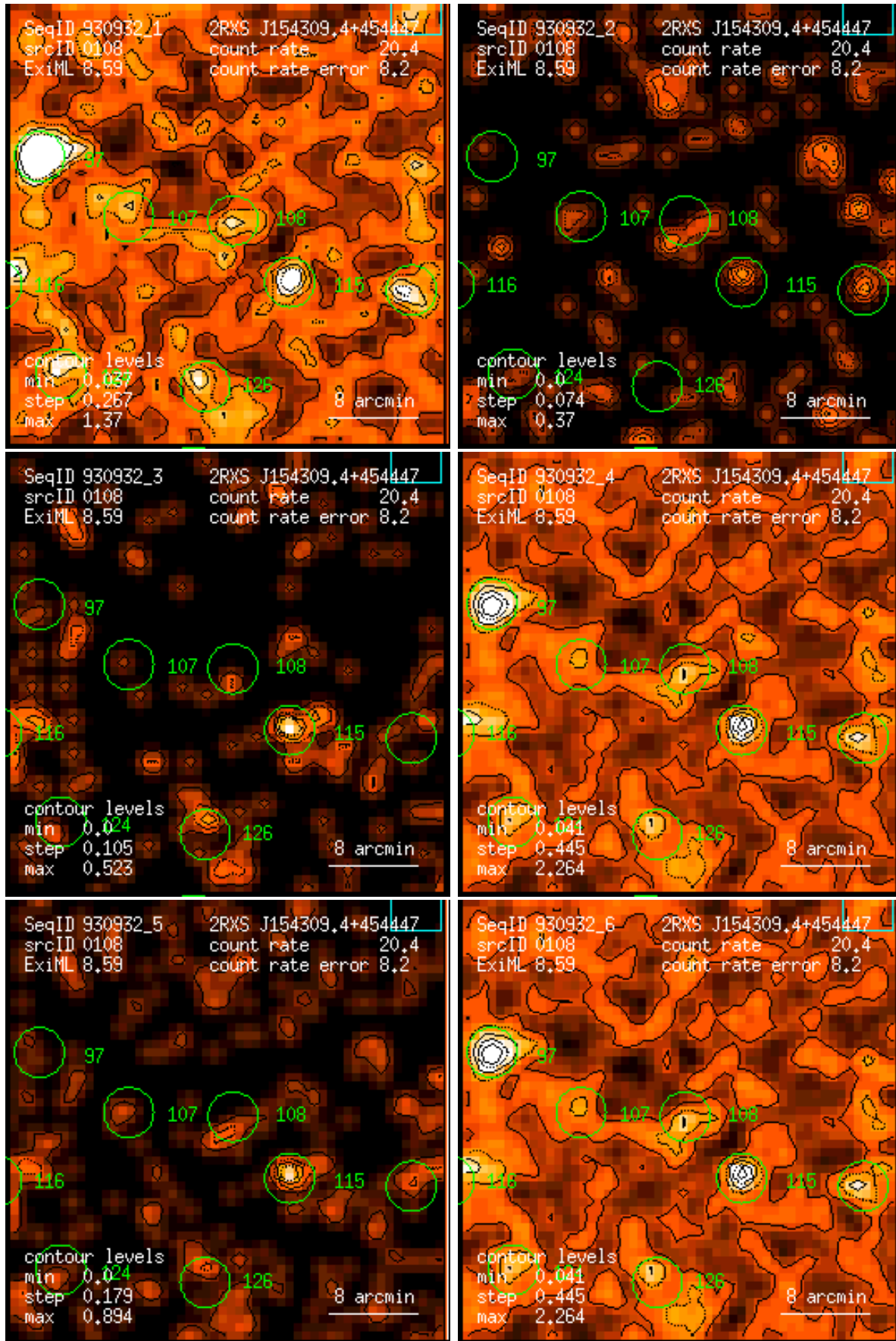
Figure 108: RASS 930932: detection 0108: band rate images, Gaussian filter: (1) PSPC channels 11 – 41, (2) 52 – 90, (3) 91 – 201, (4) 11 – 235, (5) 52 – 201, (6) 11 – 201. Broad band rates in counts/ks. Band rate contour levels in counts/ks/arcmin 2 .
