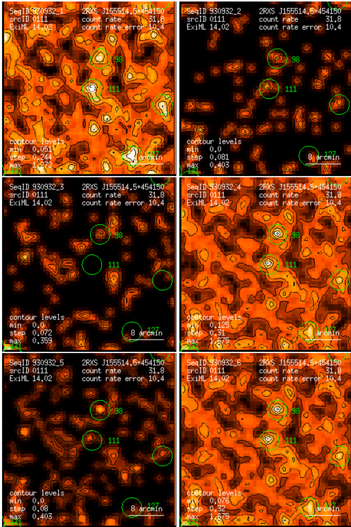
Figure 111: RASS 930932: detection 0111: band rate images, Gaussian filter: (1) PSPC channels 11 – 41, (2) 52 – 90, (3) 91 – 201, (4) 11 – 235, (5) 52 – 201, (6) 11 – 201. Broad band rates in counts/ks. Band rate contour levels in counts/ks/arcmin 2 .
