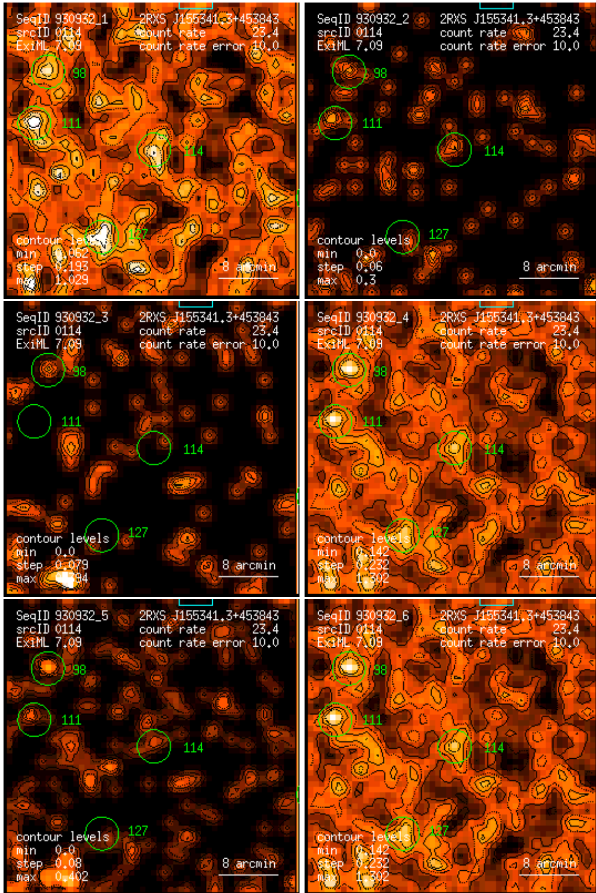
Figure 114: RASS 930932: detection 0114: band rate images, Gaussian filter: (1) PSPC channels 11 – 41, (2) 52 – 90, (3) 91 – 201, (4) 11 – 235, (5) 52 – 201, (6) 11 – 201. Broad band rates in counts/ks. Band rate contour levels in counts/ks/arcmin 2 .
