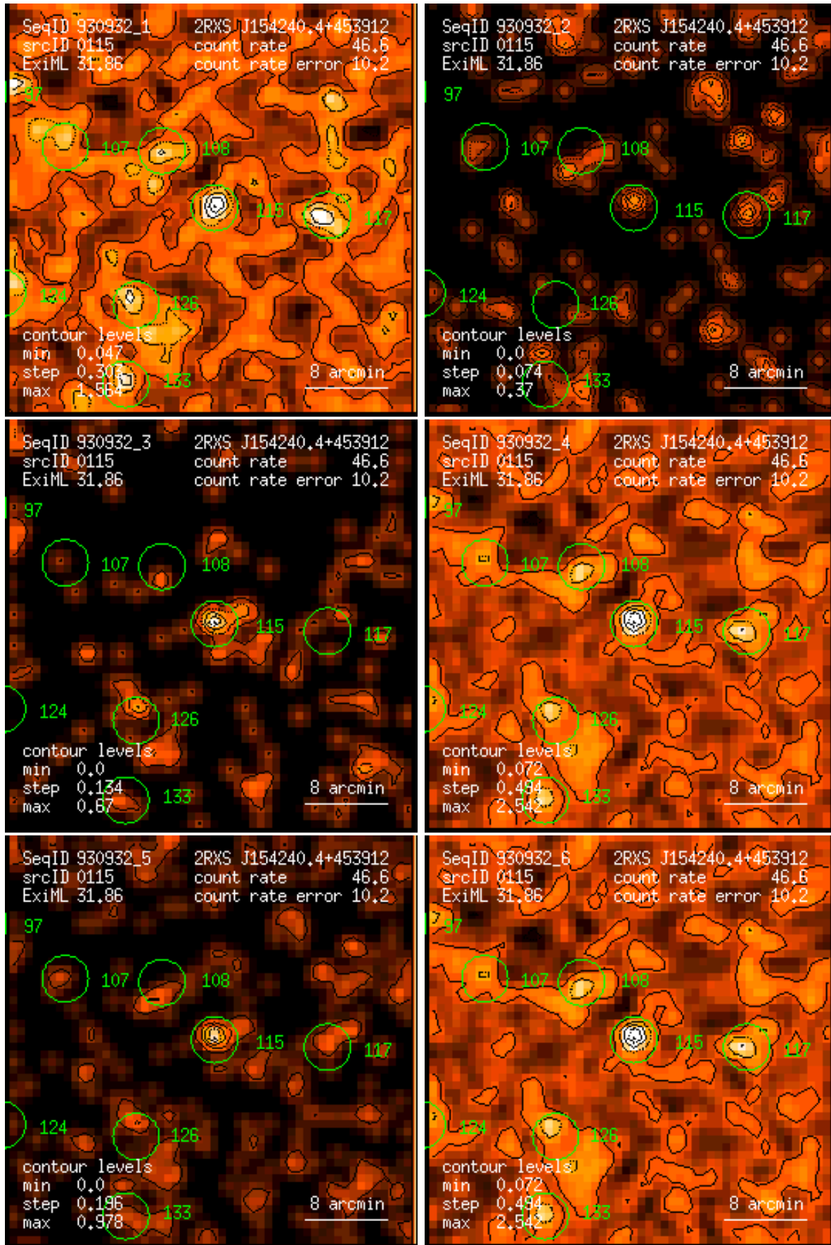
Figure 115: RASS 930932: detection 0115: band rate images, Gaussian filter: (1) PSPC channels 11 – 41, (2) 52 – 90, (3) 91 – 201, (4) 11 – 235, (5) 52 – 201, (6) 11 – 201. Broad band rates in counts/ks. Band rate contour levels in counts/ks/arcmin 2 .
