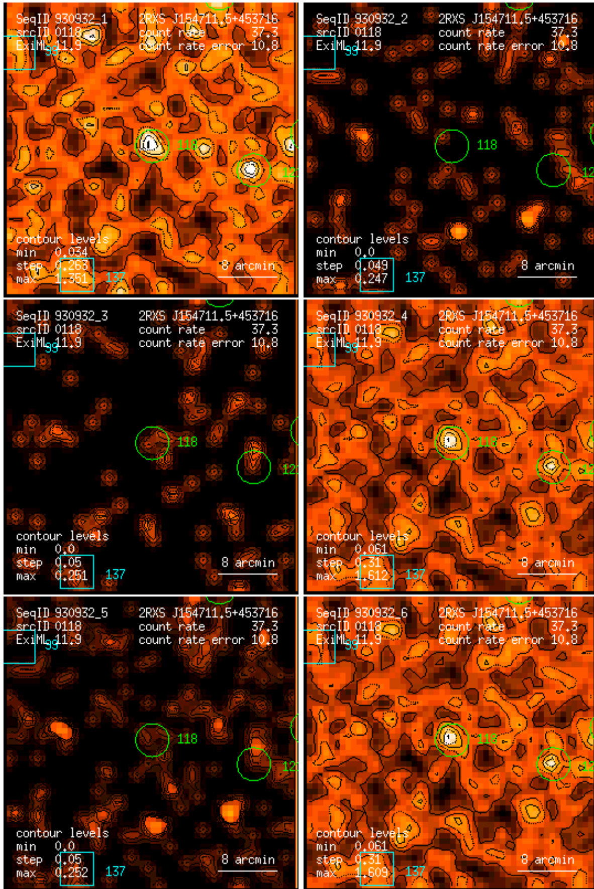
Figure 118: RASS 930932: detection 0118: band rate images, Gaussian filter: (1) PSPC channels 11 – 41, (2) 52 – 90, (3) 91 – 201, (4) 11 – 235, (5) 52 – 201, (6) 11 – 201. Broad band rates in counts/ks. Band rate contour levels in counts/ks/arcmin 2 .
