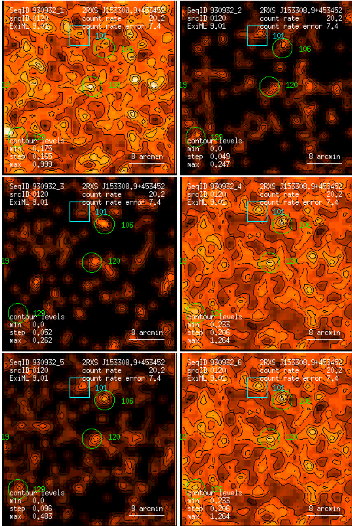
Figure 120: RASS 930932: detection 0120: band rate images, Gaussian filter: (1) PSPC channels 11 – 41, (2) 52 – 90, (3) 91 – 201, (4) 11 – 235, (5) 52 – 201, (6) 11 – 201. Broad band rates in counts/ks. Band rate contour levels in counts/ks/arcmin 2 .
